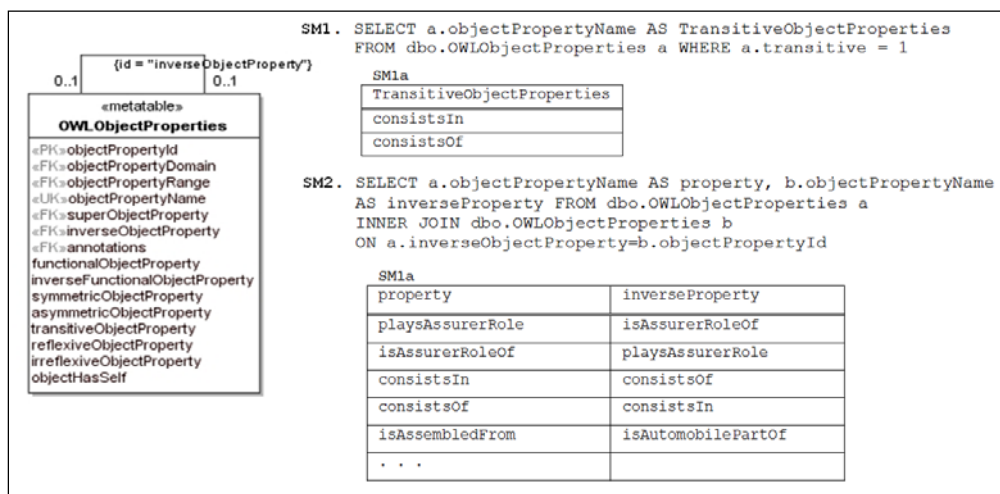
Figure 6. Example of SQL queries on metatable OWLObjectProperties (more metatables are presented in [29])
