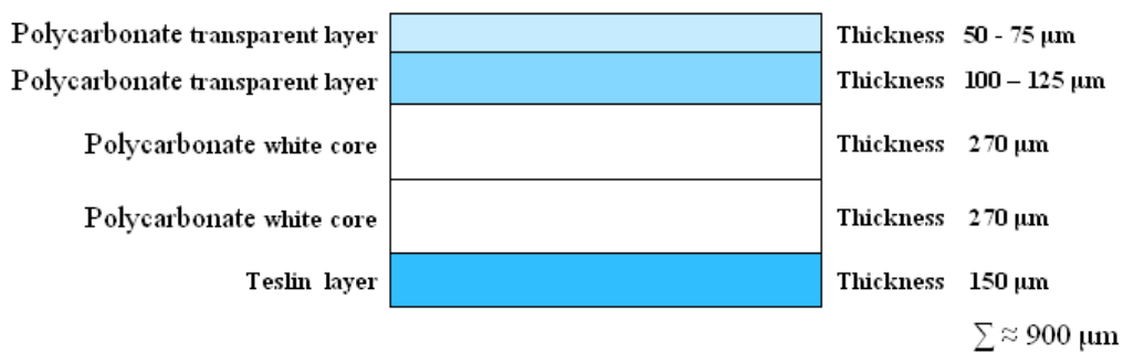
Fig. 1 Structure of the data sheet of a document formed of several polycarbonate foil layers
