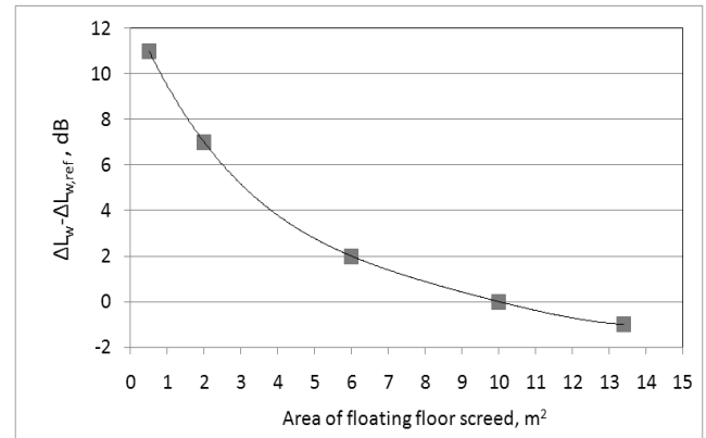
Fig. 9. The difference between determined values of \Delta L_W and reference value \Delta L_{W,ref}
