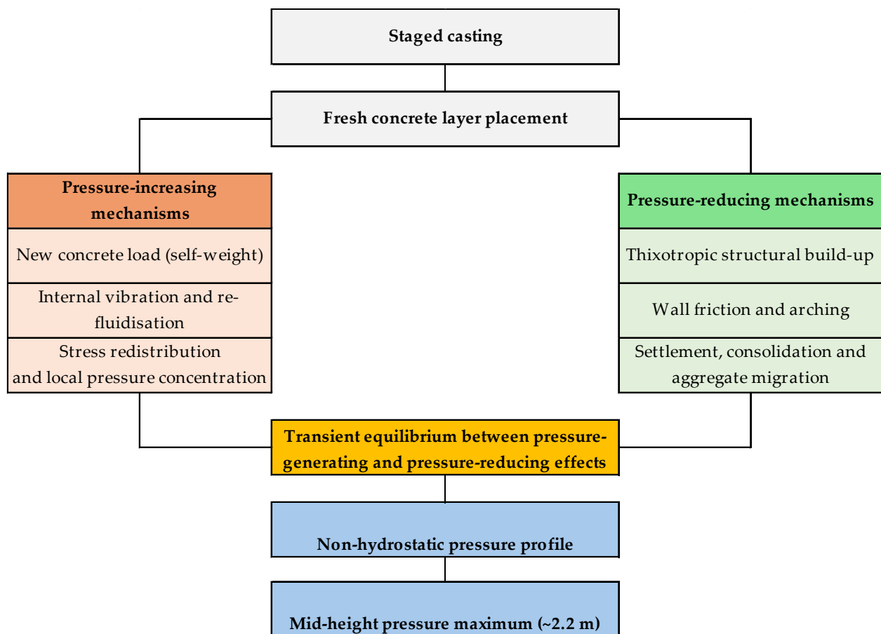
Figure 8. Conceptual framework illustrating the interaction of pressure-generating and pressure-reducing mechanisms governing fresh-concrete lateral pressure during staged casting of a single-sided wall. Pressure-generating effects include self-weight loading, vibration-induced re-fluidisation, and stress redistribution, whereas pressure-reducing effects include thixotropic structural build-up, wall friction, arching, and settlement processes. The measured non-hydrostatic pressure distribution is interpreted as reflecting a transient equilibrium between vibration-induced structural breakdown and time-dependent structural rebuilding of the concrete skeleton. The resulting pressure profile exhibits a maximum at an intermediate wall height (~2.2 m), consistent with the field measurements and the mechanistic interpretation proposed in this study. The framework is supported by previous studies on thixotropic structural build-up, vibration-induced structural breakdown, pressure redistribution, wall friction, arching, settlement, and rheological evolution of fresh concrete [2–4,6,11,12,17–19].
