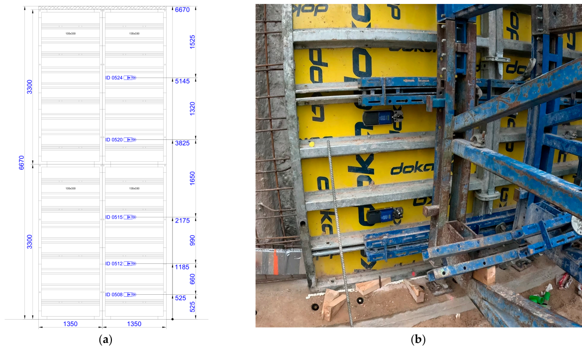
Figure 3. (a) Sensor position on the formwork; (b) view of two bottom sensors (ID 0508 and ID 0512) fixed to the formwork.
