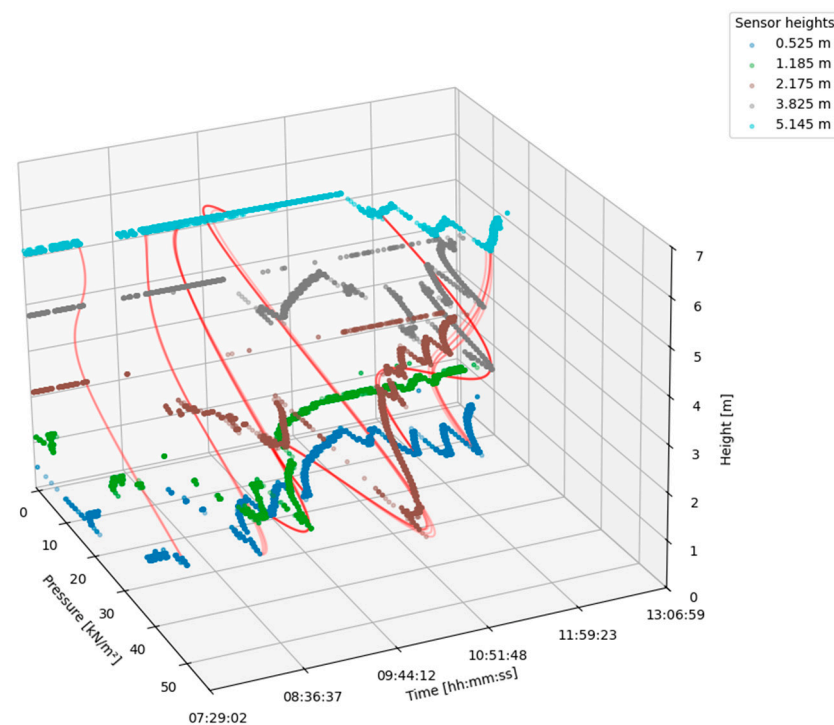
Figure 9. Raw data by sensor height, with the top-5 peak events per sensor (smoothed section curves, red). Peak pressure events are concentrated within actively vibrated zones, confirming the dominant influence of vibration.
