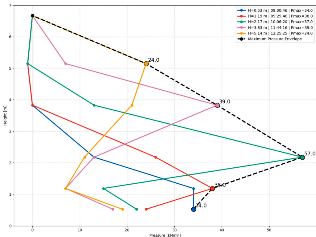
Figure 7. Envelope of maximum measured lateral pressures along the wall height. Coloured curves represent the measured pressure evolution at each sensor location. At the same time, the dashed black line denotes the maximum pressure envelope, derived from the peak value recorded at each sensor elevation. The measured peak pressure of 57 kN/m 2 occurred approximately 2.2 m above the wall base, indicating a non-hydrostatic pressure distribution and a pressure maximum located away from the wall base.
