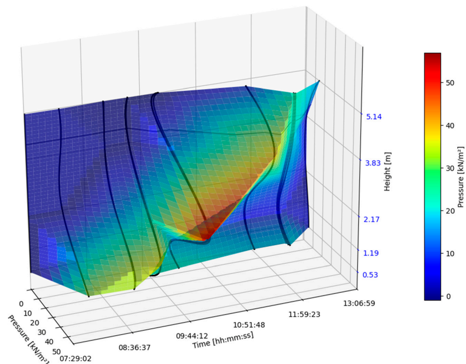
Figure 10. Pressure envelope with stretched time axis.
