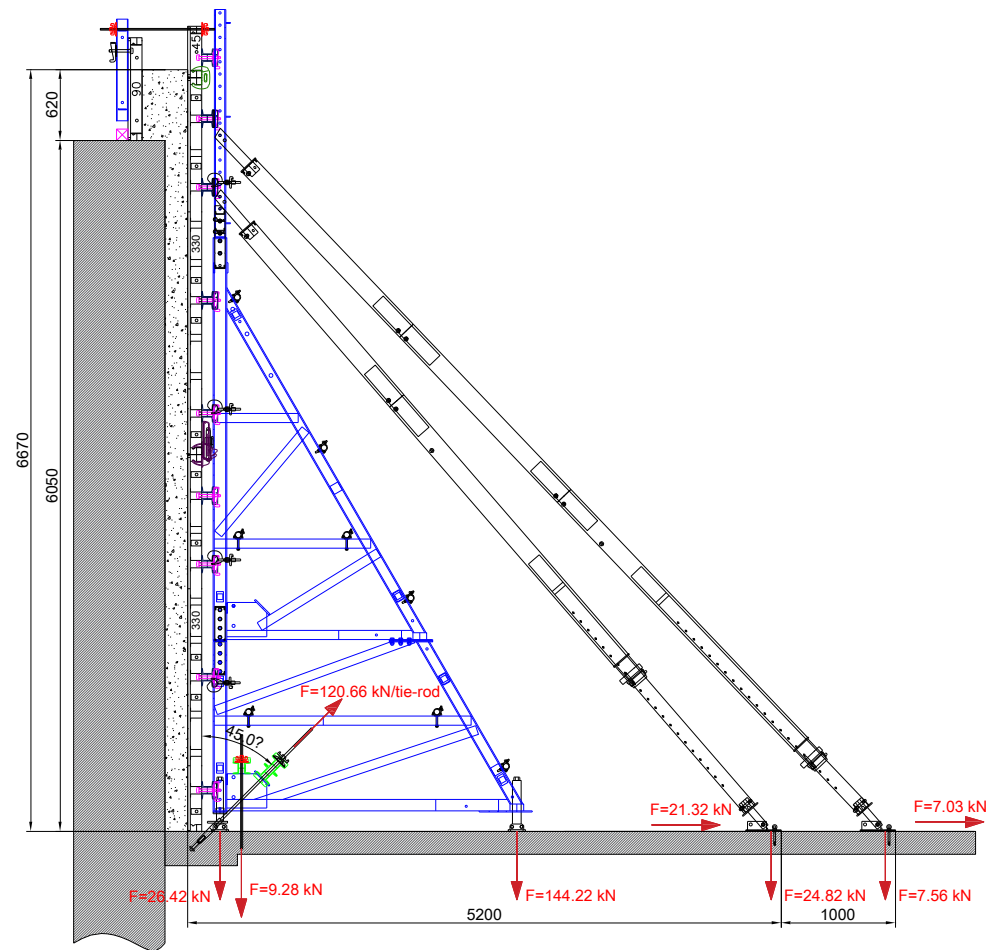
Figure 2. Formwork section with calculated acting loads.
