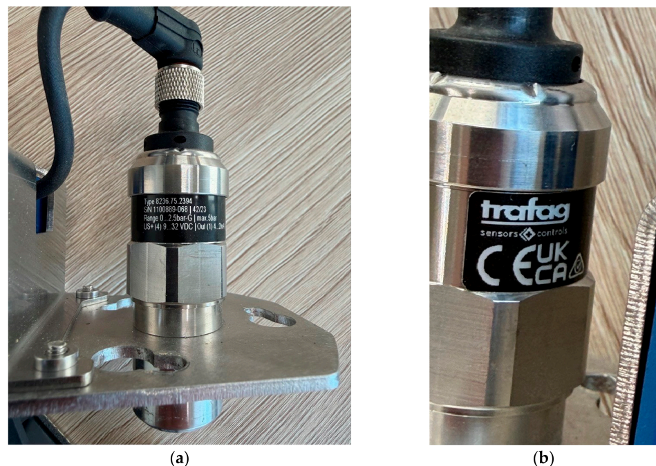
Figure 4. Trafag industrial pressure sensor: (a) sensor mounting interface view with technical characteristics; (b) sensor producer.
