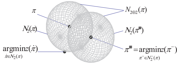
Figure 7. Graphical representation of the neighbourhood N_{2\oplus 2}
