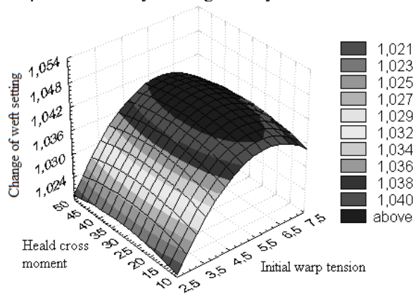
Fig. 3. The dependence of change of weft setting of half-wool fabric on initial warp tension and heald cross moment
