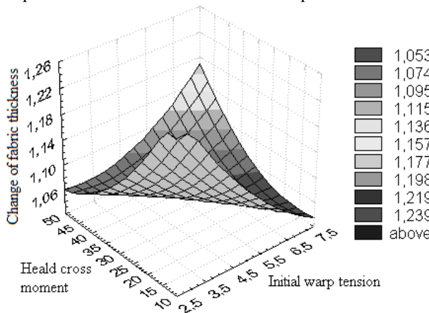
Fig. 4. The dependence of change of fabric thickness of half-wool fabric on initial warp tension and heald cross moment
