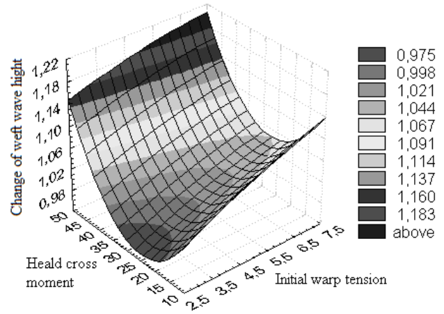
Fig. 7. The dependence of change of weft wave height on initial warp tension and heald cross moment
