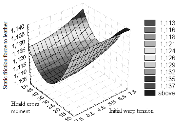
Fig. 10. The dependence of static friction force to leather on warp initial tension and heald cross moment
