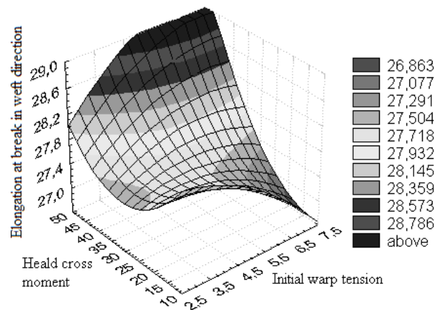
Fig. 9. The dependence of elongation at break in weft direction on warp initial tension and heald cross moment
