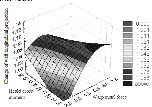
Fig. 5. The dependence of change of weft longitudinal projection on initial warp tension and heald cross moment
