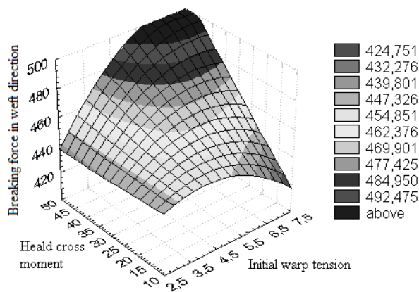
Fig. 8. The dependence of breaking force in weft direction on initial warp tension and heald cross moment
