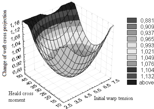
Fig. 6. The dependence of change of weft cross projection on initial warp tension and heald cross moment
