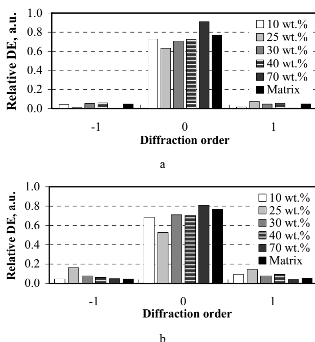
Fig. 7. Measured (a) and theoretical (b) DE distributions of replicated periodical structure vs. UA content in TMPETA/UA composition
