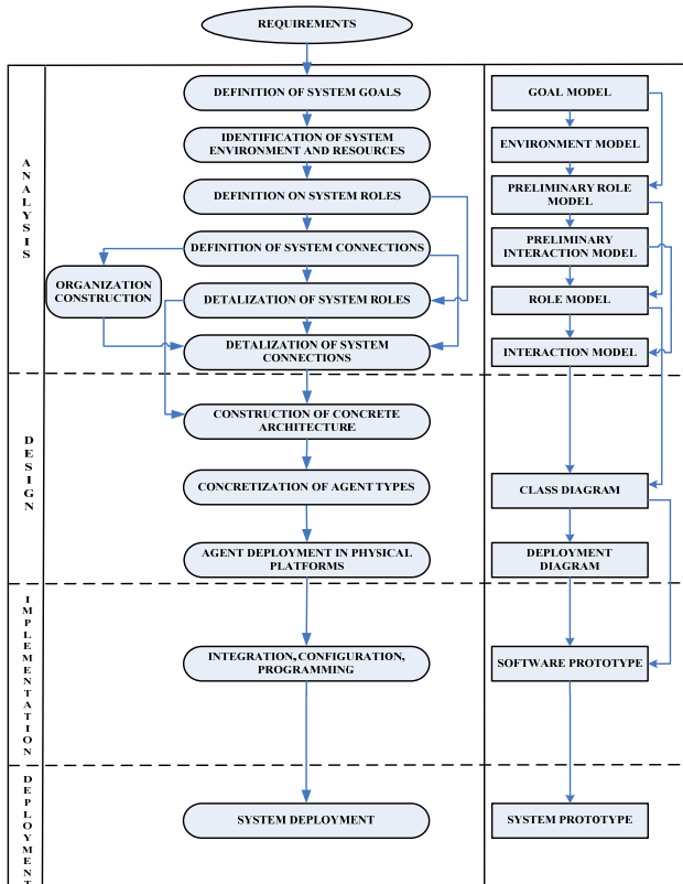
Fig. 2 Intelligent embedded system design methodology
