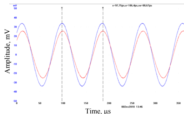
Fig. 12 Measured time response of drill-tip during tool excitation at 12 kHz frequency
