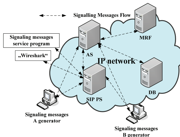
Fig. 1. Network scheme that was used during the experiment
