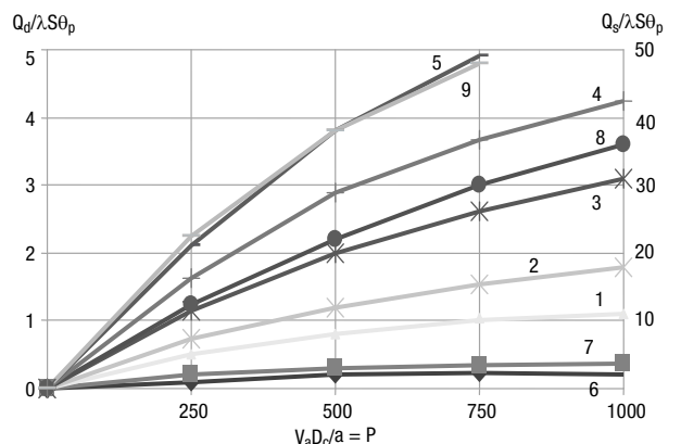
Fig. 1. The dependence of the cutting mode on the quantity of heat transferred to the detail and chip, where 1, 2, 3, ..., 9 – experiments performed
