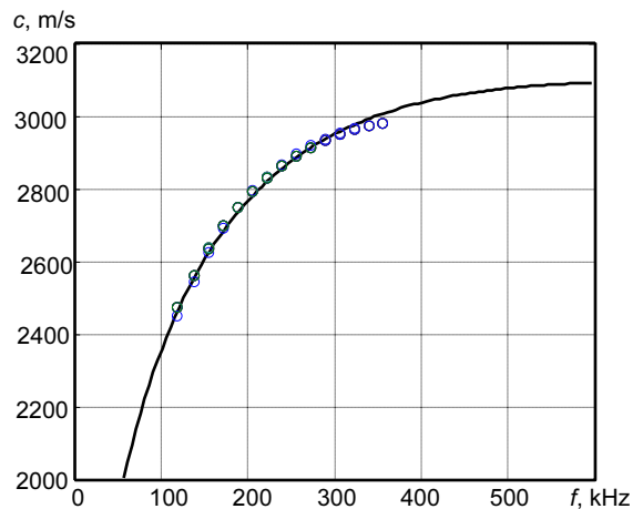
Fig.8. The theoretical dispersion curve (line) of the A_0 mode group velocity and the obtained results (circles) from simulated signals
