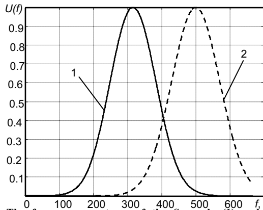
Fig.9. The frequency spectrum of the S_0 mode (1) and (2) the frequency response of the filter
