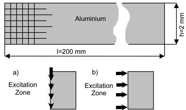
Fig.3. The finite element model for investigation of the A_0 (a) and S_0 (b) modes of the Lamb waves propagating in aluminium plate
