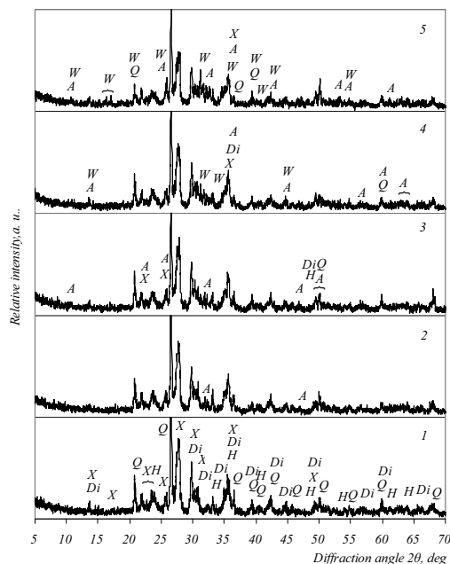
Fig. 7. X-ray diffraction patterns of Girininkai clay body (1) and clay body with MBM BA additive fired at 1025 °C for 1 h. Amount of additive: 2 – 3 %, 3 – 7 %, 4 – 10 %, 5 – 20 %. Indexes: Q – quartz, H – hematite, X – anorthite, Di – diopside, A – hydroxylapatite, W – whitlockite
