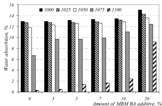
Fig. 6. Dependence of the water absorption of clay body on the amount of MBM BA additive
