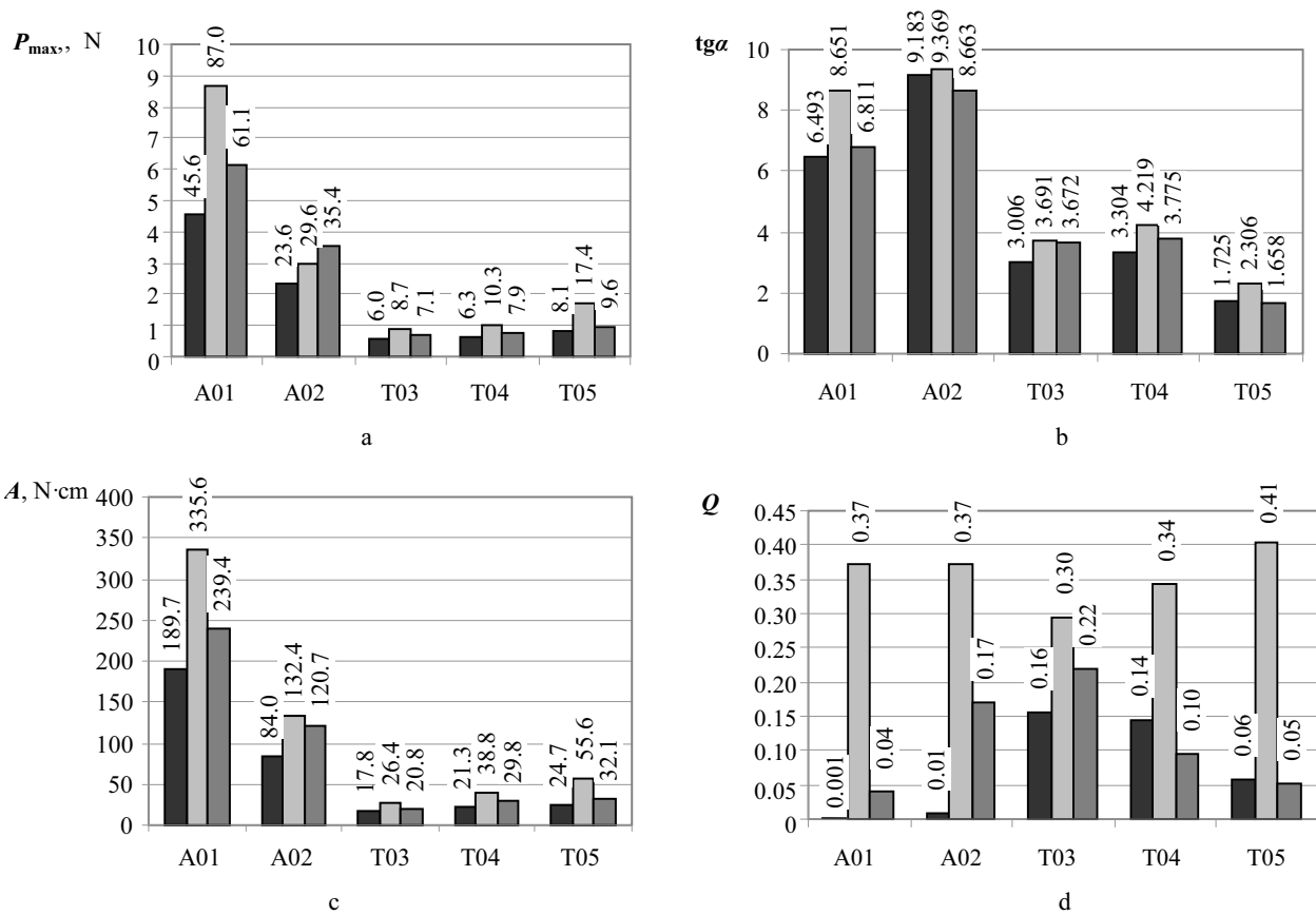
Fig. 2. The hand parameters P_{max} (a), tg\alpha (b), A (c) and Q (d) of washed and washed with followed chemical softening of woven fabrics A01, A02 and knitted materials T03, T04 and T05: ■ – control, ■ – washed, ■ – washed+softened
