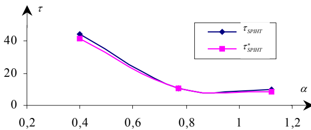
Figure 5. Impact of image smoothness on the efficiency of SPIHT encoders
