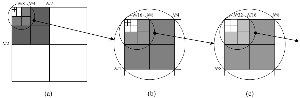
Figure 2. Generation of binary codes V(k_1, k_2) for the descendants of Y(k_1, k_2) ( k_1, k_2 \in \{0, 1, \dots, N/4-1\} ): (a) Binary codes U(k_1, k_2) , associated with wavelet coefficients in the dark-grey region, are used to generate binary codes V(k_1, k_2) , associated with wavelet coefficients in the lighter-grey region; (b) – (c) Binary codes U(k_1, k_2) and V(k_1, k_2) in the dark-grey regions are used to generate binary codes V(k_1, k_2) in the lighter-grey regions
