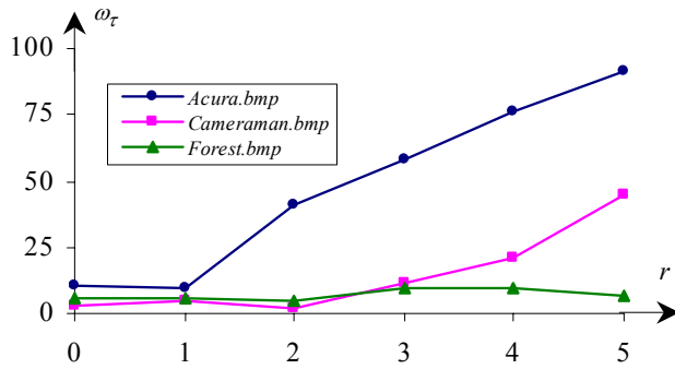
Figure 4. Image encoding speed gains (lossless and lossy image compression)
