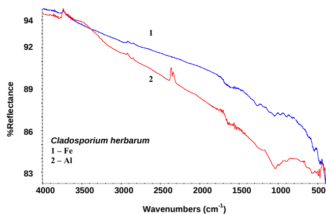
Fig. 6. FTIR spectra of steel and Al specimens exposed to Cladosporium herbarum fungi for 30 days
