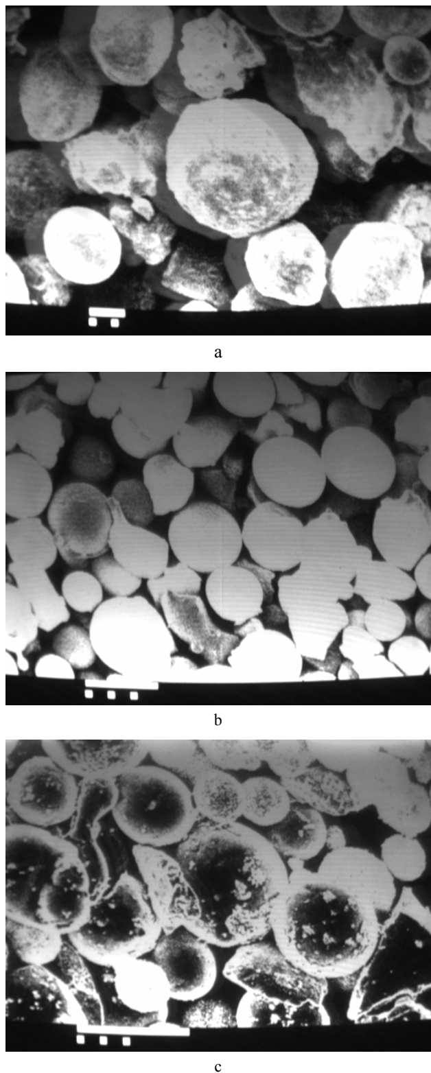
Fig. 1. SEM pictures of powders used for thermal spray process: a – WC-Co (mark length 10 \mu\text{m} ); b – Cr 2 C 3 -NiCr (mark length 100 \mu\text{m} ); c – WC-Co/NiCrBSi (mark length 100 \mu\text{m} )
