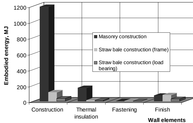
Fig. 8. Embodied energy of masonry and straw bale construction
