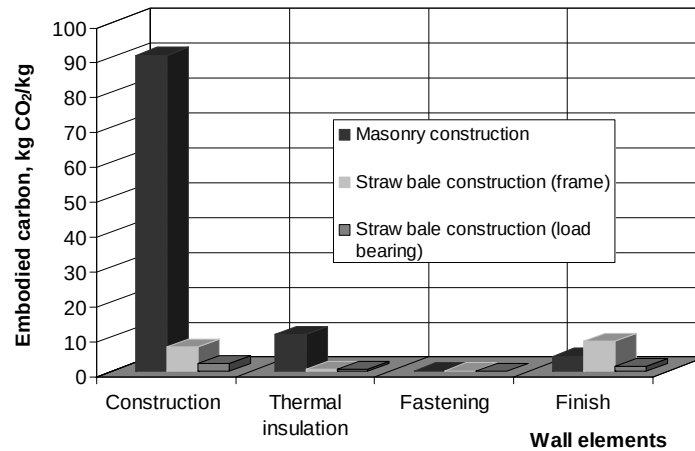
Fig. 9. Embodied carbon of masonry and straw bale construction
