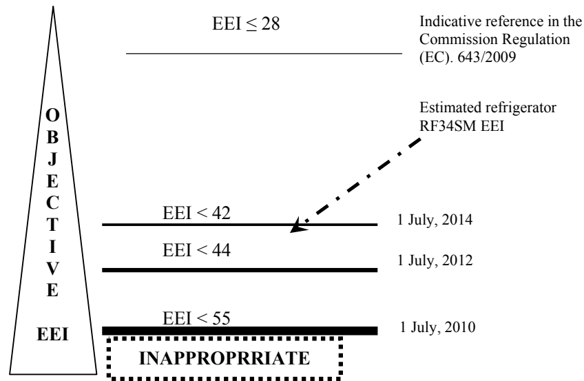
Fig. 2. Legal requirements for energy efficiency (EEI) and the refrigerator/freezer RF34SM EEI
