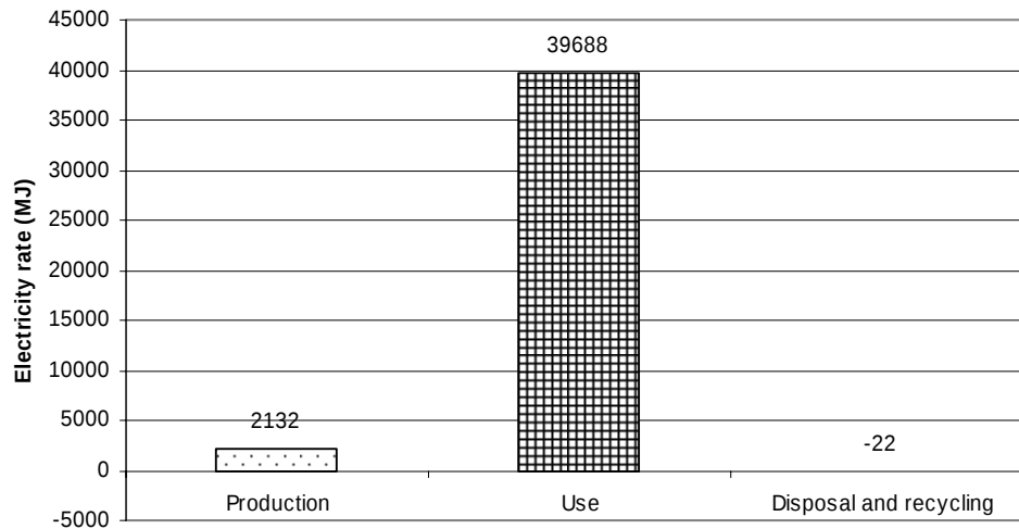
Fig. 1. Electricity consumption during the overall refrigerator/freezer life-cycle
