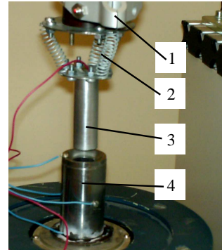
Fig. 3. Initial state of the parts in assembly position before the joining: 1 – robot gripper; 2 – remote center compliance device; 3 – shaft; 4 – bushing
