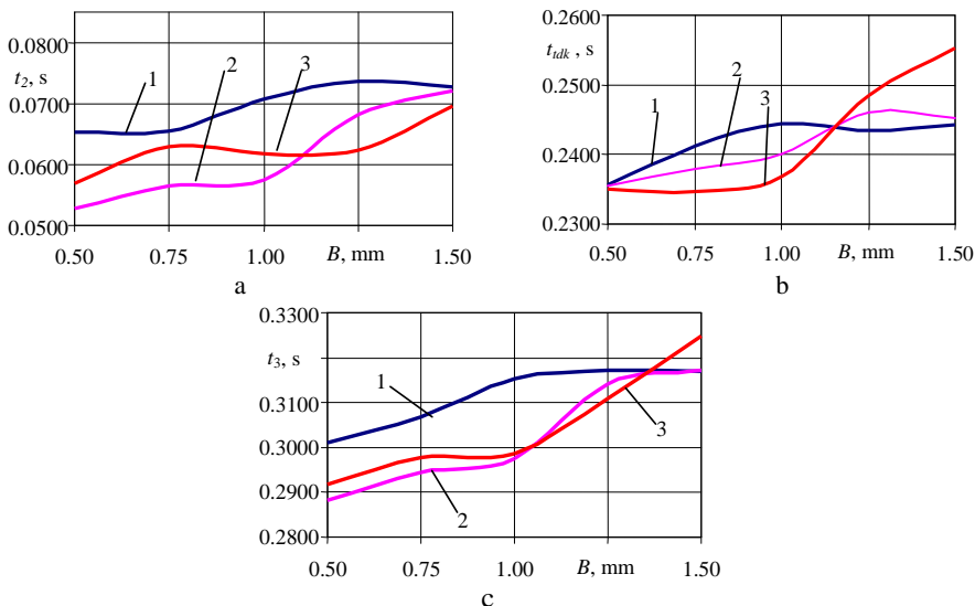
Fig. 13 Dependences of: a – duration t_2 ; b – two point contact stage duration t_{dk} ; c – insertion process duration t_3 , on excitation amplitude B , excitation frequency: 1 – f = 50 Hz; 2 – f = 70 Hz; 3 – f = 100 Hz
