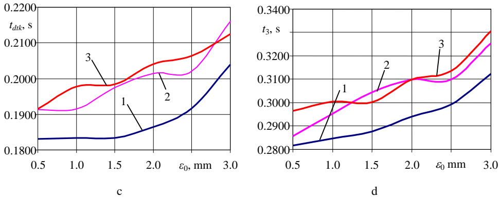
Fig. 15. Dependences of: a – chamfer crossing duration t_1 ; b – duration t_2 , from the beginning of insertion process until the beginning of two-point contact stage; c – two-point contact stage duration t_{dk} ; d – insertion process duration t_3 , on lateral positioning error of the shaft \varepsilon_0 , when \theta_0 = 0.0175 rad, 1 – without vibratory excitation; 2 – exciting vibrations of the bushing with the frequency f_2 = 70 Hz and amplitude B = 1.0 mm; 3 – f = 70 Hz, B = 1.5 mm
