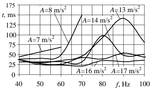
Fig. 5. Dependences of alignment time t versus the excitation frequency f , as pressing force F=9.81 N, axial misalignment \Delta=1.75 mm
