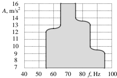
Fig. 11. Area of the reliable alignment (unhatched), depending on the amplitude A of the excitation acceleration and frequency f , when \Delta=3 mm, F=9.81 N, k=1.8 N/mm
