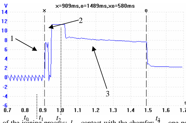
Fig. 4. Oscillogram of the joining process: 1 – contact with the chamfer; 2 – one-point contact; 3 – two-points contact
