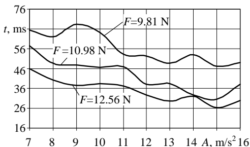
Fig. 9. Dependences of the parts alignment time t versus the acceleration amplitude of bushing's excitation, when \Delta=3 mm
