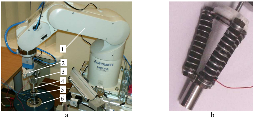
Fig. 1. Experimental setup for robotized vibratory assembly: a – general view; 1 – robot; 2 – robot gripper; 3 – remote center compliance device; 4 – shaft; 5 – bushing of particular construction; 6 – vibrator; b – remote center compliance device of adjustable rigidity
