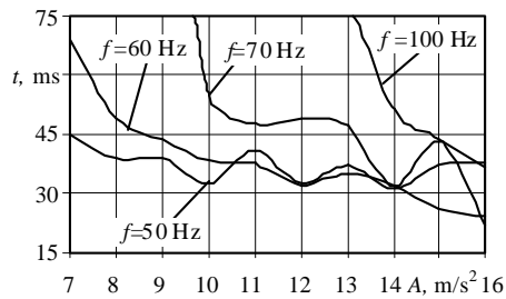
Fig. 6. Dependences of alignment time t versus the amplitude A of the excitation acceleration, as F=9.81 N, \Delta=1.75 mm
