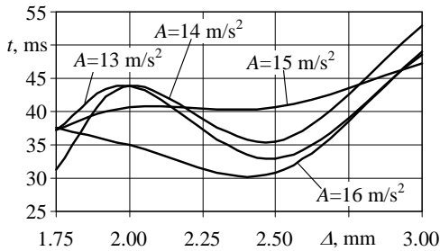
Fig. 7. Alignment time dependence on the shaft-to-bushing axial misalignment, as excitation frequency is 40 Hz, F=9,81 N
