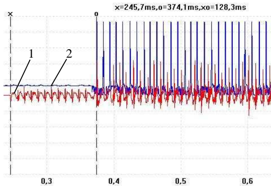
Fig. 2. Measurement scheme of the alignment duration: 1 – signal from the acceleration sensor; 2 – signal which indicates the end of alignment
