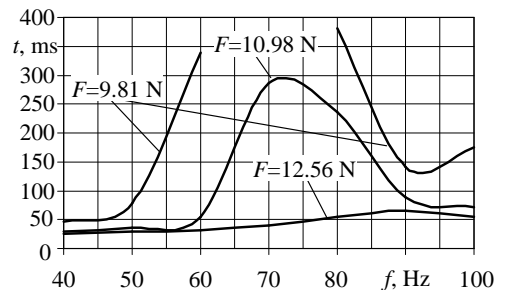
Fig. 10. Dependences of the parts alignment time t versus bushing's excitation frequency, as A=15 m/s 2 , \Delta=2 mm
