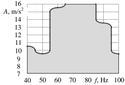
Fig. 12. Area of the reliable alignment (unhatched), depending on the amplitude A of the excitation acceleration and frequency f , when F=9.81 N, \Delta=2 mm and k=4.5 N/mm
