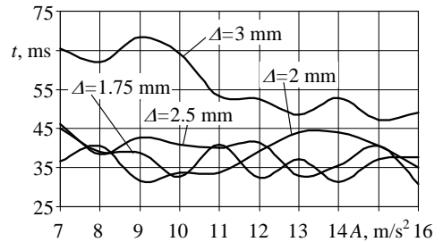
Fig. 8. Part alignment time t dependences on the amplitude A of the excitation acceleration, as F=9.81 N, f=40 Hz
