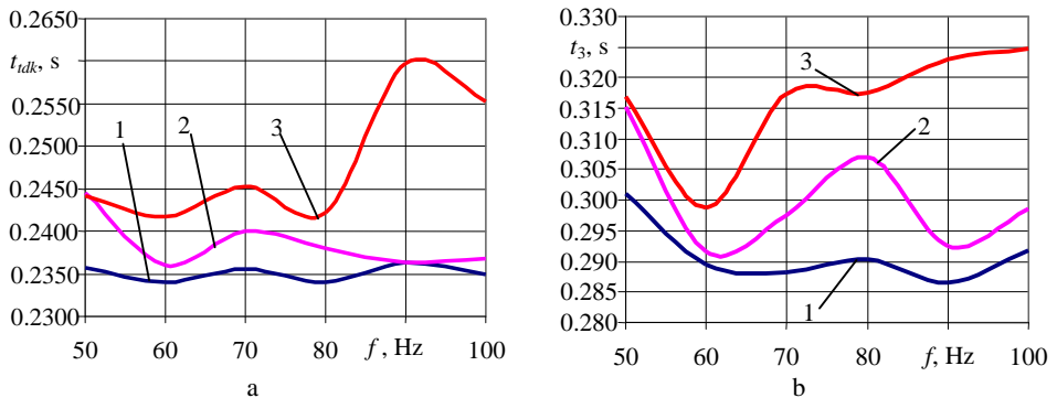
Fig. 14. Dependences of: a – two-point contact stage duration t_{dk} ; b – insertion process duration t_3 , on excitation frequency and excitation amplitudes: 1 – B = 0.5 mm; 2 – B = 1.0 mm; 3 – B = 1.5 mm
