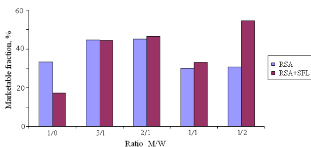
Fig. 6. Dependence of marketable fraction on molasses/water ratio
