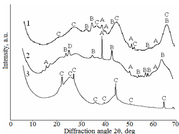
Fig. 5. X-ray diffraction patterns of: 1 – \text{Al}_2\text{O}_3\text{-C}_{\text{act}} composite, 2 – \text{Al}_2\text{O}_3 , 3 – WS-42A activated carbon. A – \text{AlO}(\text{OH}) , B – \gamma\text{-Al}_2\text{O}_3 , C – carbon, D – \text{Al}_2(\text{SO}_4)_3
