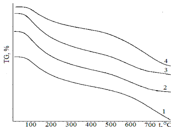
Fig. 4. TG curves of \text{Al}_2\text{O}_3\text{-C}_{\text{act}} at air atmosphere: 1 – \text{Al}_2\text{O}_3\text{-(WS-42A)} , 2 – \text{Al}_2\text{O}_3\text{-(B-2)} , 3 – \text{Al}_2\text{O}_3\text{-(WS-42)} , 4 – \text{Al}_2\text{O}_3\text{-(OU)}
