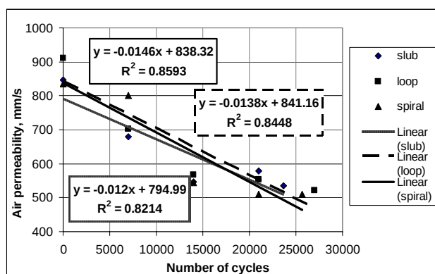
Fig. 5. The dependencies of fabrics air permeability on number of abrasion cycles for fabrics with fancy yarns of different structure
