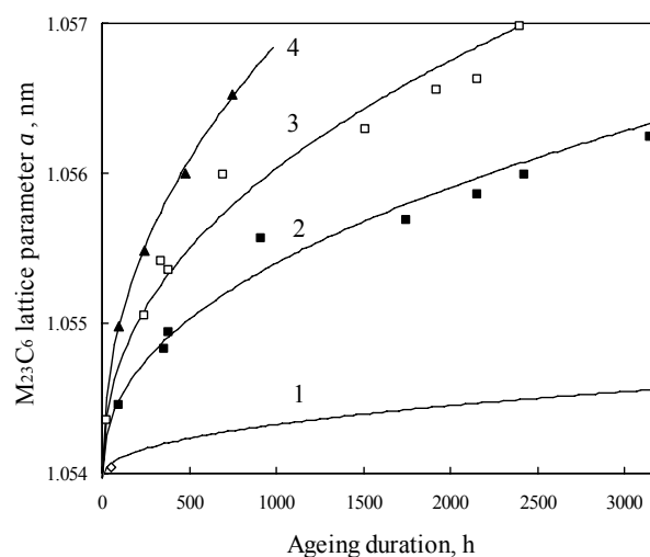
Fig. 4. The changes of lattice parameter a of carbide \text{M}_{23}\text{C}_6 in 12X1MΦ steel depending on ageing time in service conditions – 1, ageing at 2 – 600 °C, 3 – 650 °C and 4 – 700 °C temperature
