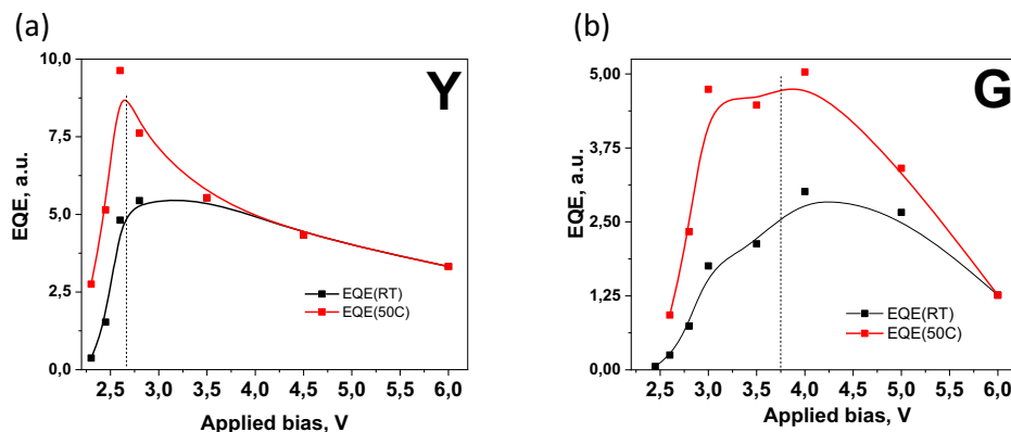
Fig. 7 | Calculated relative EQE values as a function of applied bias. (a) Y and (b) G devices at room temperature (black symbols) and 50 °C (red symbols); solid curves are the guide for the eye. The vertical dashed lines in the graphs mark the maximal values of EQE at high temperature, which are close to the isosensitive points shown in Fig. 6.
