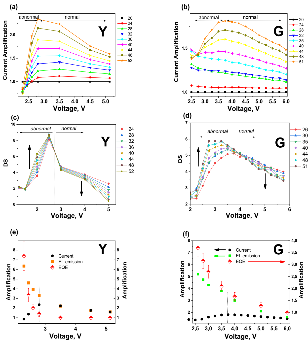
Fig. 6 | Effect of temperature on the OLED performance. a, b Amplification of the current at the indicated temperature (shown in the legend in °C) relatively to the current at room temperature as a function of the applied bias; (c, d) DS as a function of applied bias at the indicated temperature (shown in the legend in °C) and (e, f)
