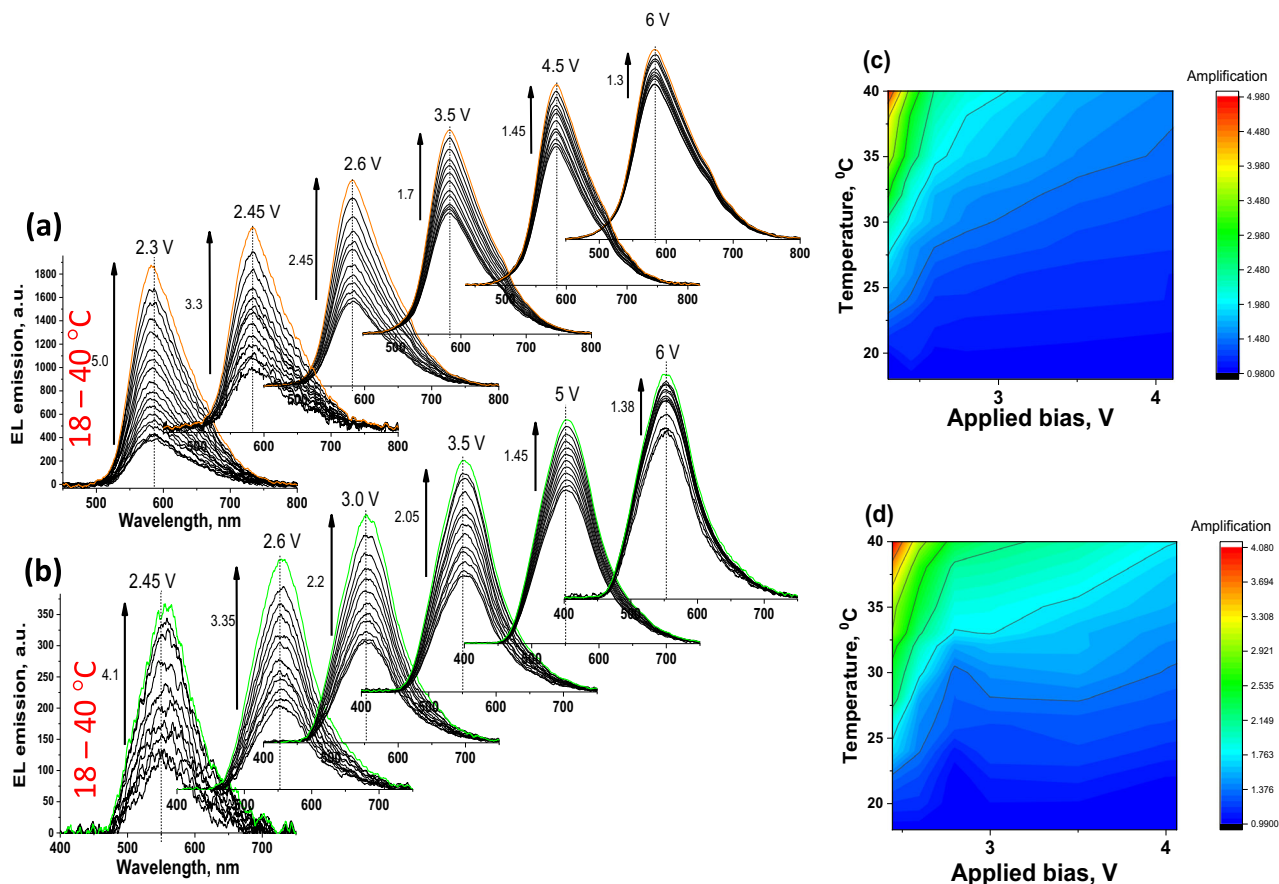
Fig. 4 | Thermal enhancement of the OLED emission. a, b EL spectra and (c, d) 3D maps of the relative increase of EL emission as a function of the applied voltage and increasing temperature relative to that at room temperature: (a, c) Y device and (b, d)
