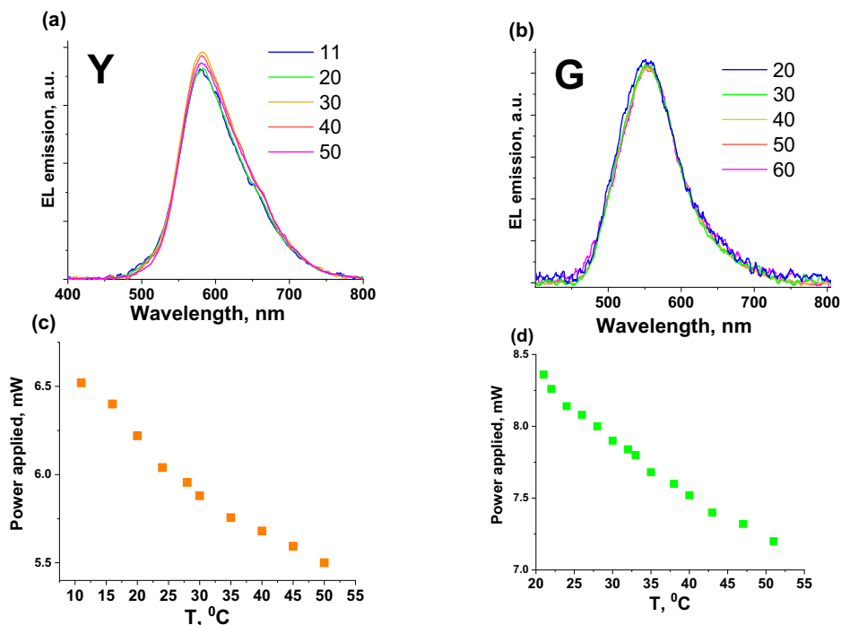
Fig. 8 | Enhancement of power efficiency of the OLEDs. a, b EL emission spectra and (c, d) power consumed by the OLEDs as a function of temperature under a constant current regime of 2 mA for (a, c) Y device and (b, d) G device. In (a, b) the temperature is indicated in the legend in °C.
