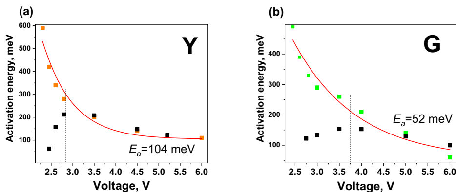
Fig. 9 | Activation energy for EL (yellow and green symbols) and for carrier injection (black symbols) as a function of applied bias. (a) Y device and (b) G device. The vertical dashed line corresponds to the isosensitive point that separates normal and abnormal regions.
