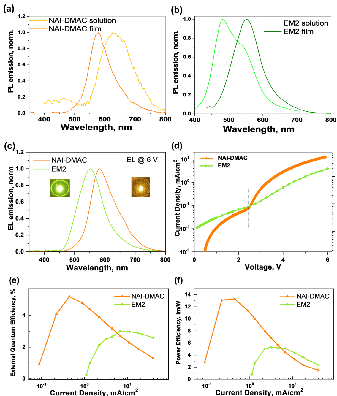
Fig. 3 | Basic characteristics of the TADF emitters and OLED devices. PL emission spectra of dye solutions ( 10^{-5} M) and films of (a) NAI-DMAC and (b) EM2; c normalized EL spectra at applied bias of 6 V (insert shows visual emission of the Y
