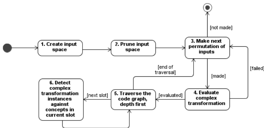
Figure 10. An algorithm for detecting how complex transformation relates parts of program model with parts of program code
