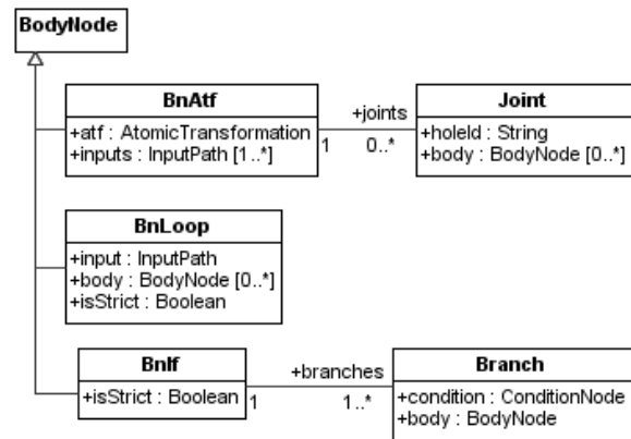
Figure 6. Model of a complex transformation body
