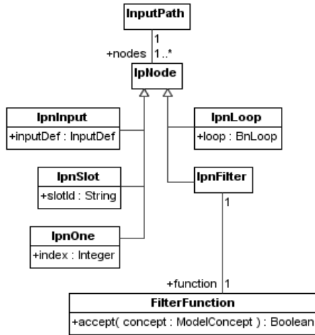
Figure 7. Model of input paths
