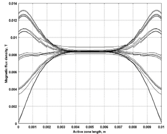
Fig. 3. Simulation results of magnetic flux density in the active cylinder zone for middle poles inductor for the each time step. The active zone is limited by relative diameter D_a / D = 1
