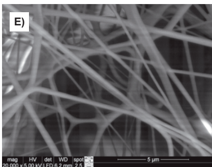
Figure 5. SEM images of nonwoven webs formed from 7 wt.% PVA solutions and 5 % ethanol containing various starch amounts at 65 kV applied voltage. A – 1% starch (scale 5 µm), B – 1% starch (scale 200 µm), C – 3% starch (scale 5 µm), D – 3% starch (scale 200 µm), E – 5% starch (scale 5 µm), F – 5% starch (scale 200 µm) in the polymer solution, (1 – fibres of support material, 2 – nanofibres, 3 – spots of polymer solution).
