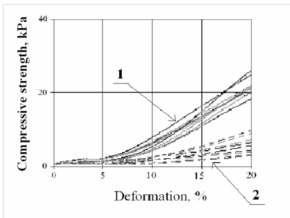
Fig. 6. Compressive strength curves comparison of wool: 1 – “A” type specimen; 2 – “B” type specimen
