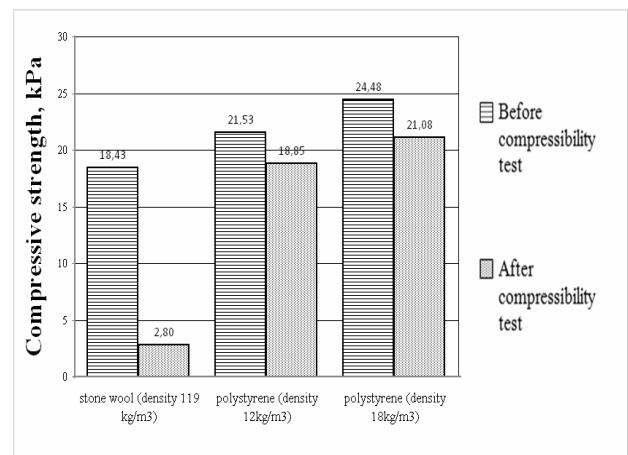
Fig. 4. Comparison of compressive strength values of 40 mm thickness specimens
