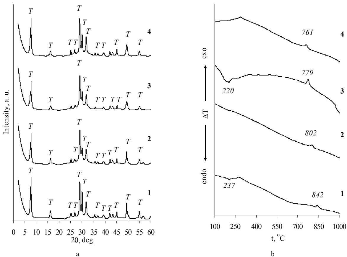
Fig. 6. XRD patterns (a) and DSC curves (b) of synthesis products from CaO and amorphous silica mixtures with \gamma\text{-Al}_2\text{O}_3 additive when synthesis duration is 8 h. Amount of \text{Na}_2\text{O} added, %: 1 – 0; 2 – 1; 3 – 5; 4 – 10. Indexes: T – 1.13 nm tobermorite
