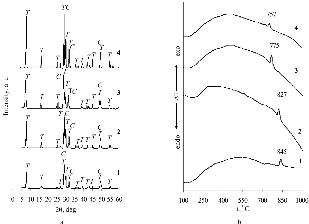
Fig. 5. XRD patterns (a) and DSC curves (b) of synthesis products from CaO and amorphous silica mixtures with \gamma\text{-Al}_2\text{O}_3 additive when synthesis duration is 4 h. Amount of \text{Na}_2\text{O} added, %: 1 – 0; 2 – 1; 3 – 5; 4 – 10. Indexes: T – 1.13 nm tobermorite, C – C-S-H(I)
