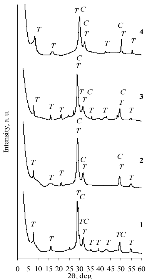
Fig. 3. XRD patterns of synthesis at 175 °C temperature products from CaO and SiO 2 ·nH 2 O mixtures when duration of curing is 24 h and Na 2 O additive content, %: 1 – 0; 2 – 1; 3 – 5; 4 – 10. Indexes: T – 1.13 nm tobermorite, C – C-S-H(I)
