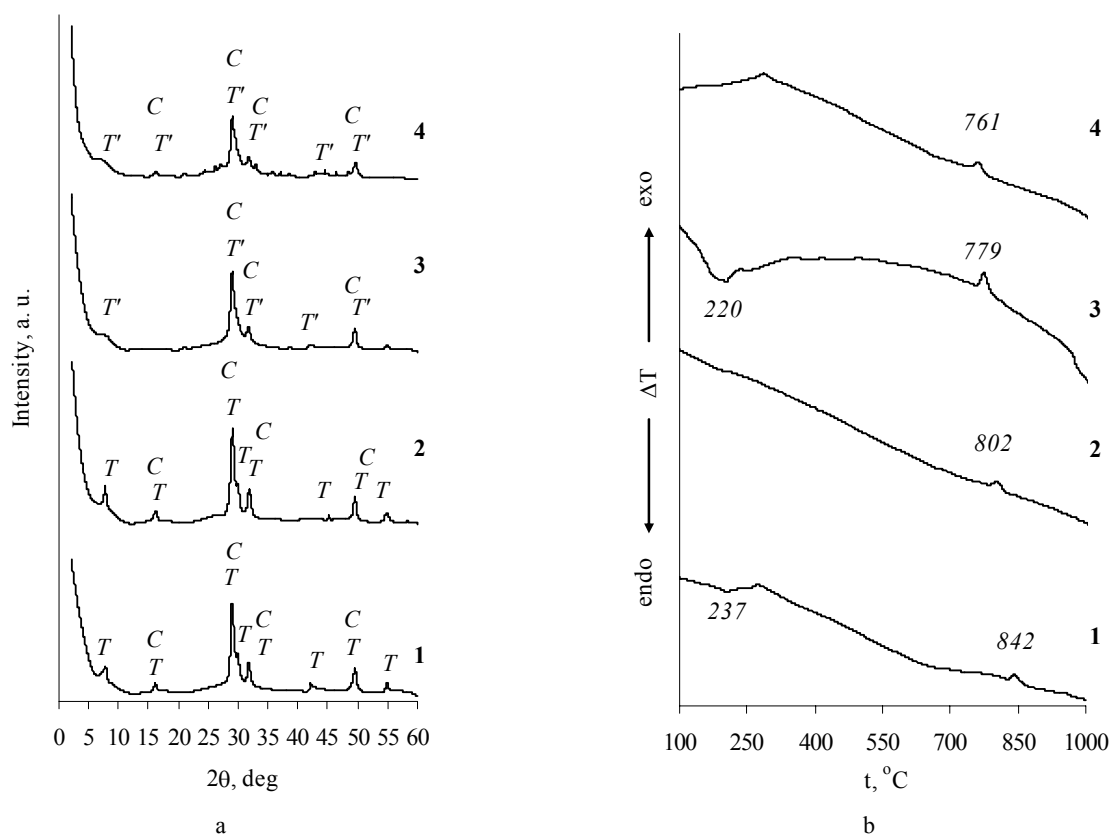
Fig. 2. XRD diffraction patterns and DSC curves of synthesis products from \text{CaO-SiO}_2 \cdot n\text{H}_2\text{O} mixtures. Temperature – 175^\circ\text{C} when duration of curing is 16 h and \text{Na}_2\text{O} content, %: 1 – 0; 2 – 5; 3 – 7; 4 – 10. Indexes: C – C-S-H(I), T' – tobermorite gel, T – 1.13 nm tobermorite
