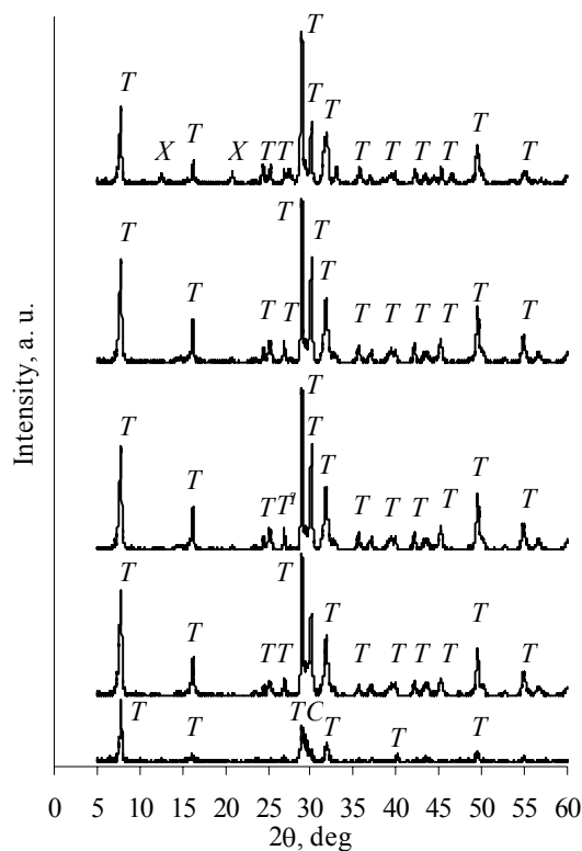
Fig. 7. XRD diffraction patterns of synthesis products at 175 °C temperature, when composition of initial mixtures \text{C/(S+A)}=0.083 , amount of additives and synthesis duration: 1 – \text{A/(S+A)}=0 , \text{Na}_2\text{O}=0\% , \tau=24 h; 2 – \text{A/(S+A)}=0.025 , \text{Na}_2\text{O}=0\% , \tau=24 h; 3 – \text{A/(S+A)}=0.025 , \text{Na}_2\text{O}=5\% , \tau=24 h; 4 – \text{A/(S+A)}=0.025 , \text{Na}_2\text{O}=0\% , \tau=32 h; 5 – \text{A/(S+A)}=0.025 , \text{Na}_2\text{O}=5\% , \tau=32 h. Indexes: T – 1.13 nm tobermorite, C – C-S-H(I), X – xonotlite
