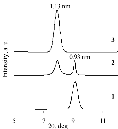
Fig. 9. Thermal type of tobermorite. XRD patterns after 3 h heating at 300 °C temperature. Duration of synthesis – 24 h and composition of initial mixtures: 1 – C/S=0.83, Na 2 O=0 %; 2 – C/(S+A)=0.83 ir A/(S+A)=0.025, Na 2 O=0 %, 3 – C/(S+A)=0.83 ir A/(S+A)=0.025, Na 2 O=5 %
