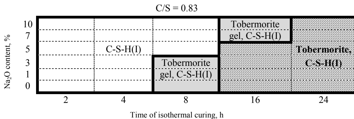
Fig. 4. Influence of sodium oxide quantity and duration of synthesis at 175 °C temperature on the mineral composition of products
