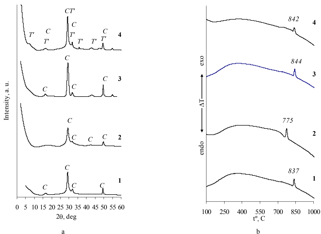
Fig. 1. XRD patterns (a) and DSC curves (b) of synthesis products, when duration of curing and \text{Na}_2\text{O} content: 1 – 2 h, \text{Na}_2\text{O} = 0\% ; 2 – 2 h, \text{Na}_2\text{O} = 5\% ; 3 – 4 h, \text{Na}_2\text{O} = 0\% ; 4 – 8 h, \text{Na}_2\text{O} = 0\% . Indexes: C – C-S-H(I); T' – tobermorite gel
