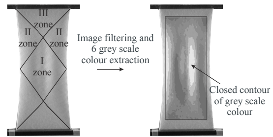
Fig. 2. The principle of image analysis for specimen buckling moment evaluation (unstitched specimen elongation 4 %)
