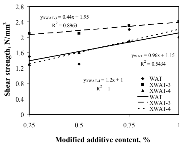
Fig. 2. Dependence of the bond strength of samples glued at 20 °C with PVA DP51/10 dispersion on the type of modifying additive: ♦ – DP51/10 + WAT; ■ – DP51/10 + XWAT-3; ▲ – DP51/10 + XWAT-4
