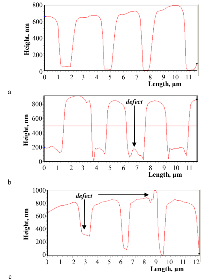
Fig. 7. AFM images and profiles of embossed periodical structures vs photopolymer type and effective initial UV curing duration \tau , s: a – PHP I (10 s); b – PHP II (20 s); c – PHP III (30 s)
