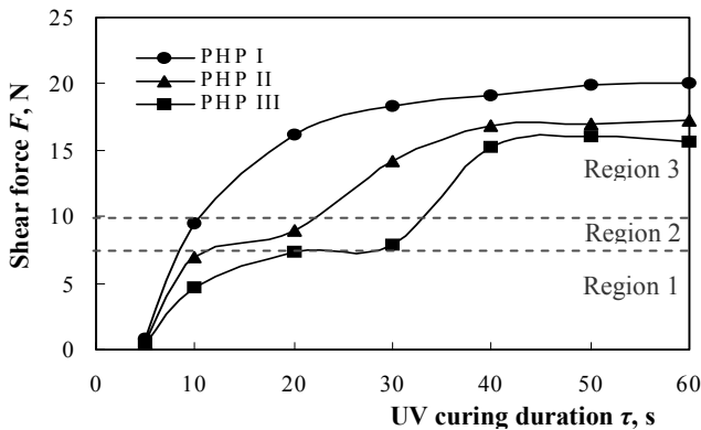
Fig. 5. The scratch resistance of polymeric layers vs UV curing duration and photopolymer type
