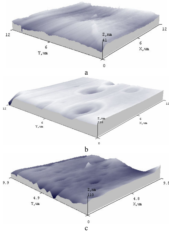
Fig. 6. AFM images and profiles of photopolymer coatings surface structure vs photopolymer type: a – PHP I; b – PHP II; c – PHP III
