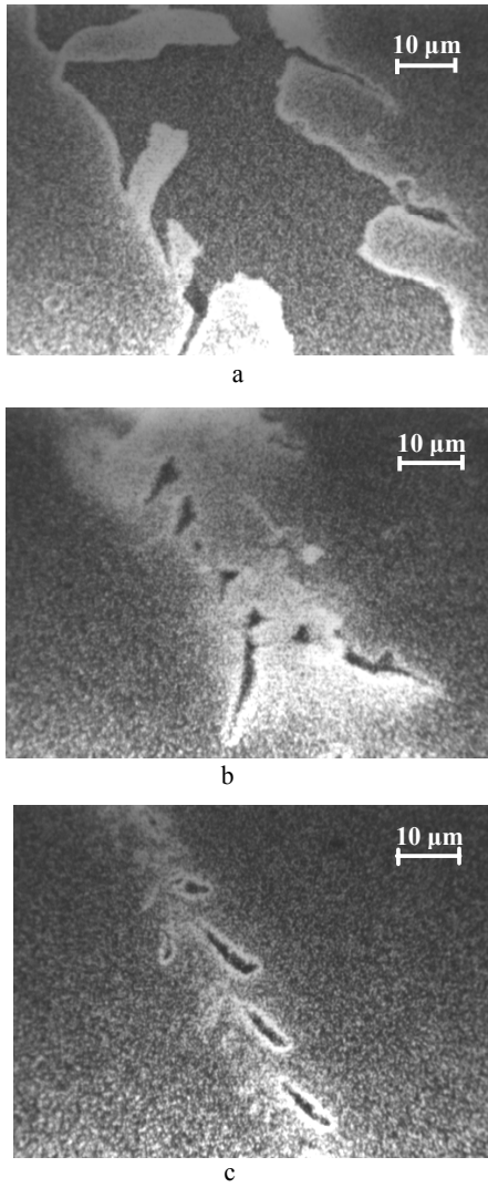
Fig. 4. SEM images of scratch groove ( P_n = 100 mN) for PHP I coating cured at different durations: a – 5 s; b – 10 s; c – 20 s
