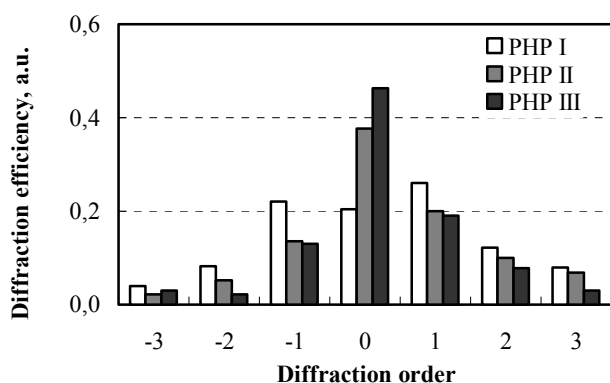
Fig. 8. Relative diffraction efficiency of replicated periodical structures vs photopolymer type
