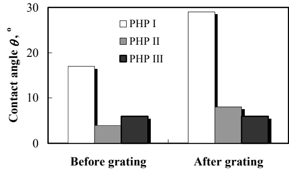
Fig. 3. The variation of contact angle vs photopolymer type and Ni surface roughness
