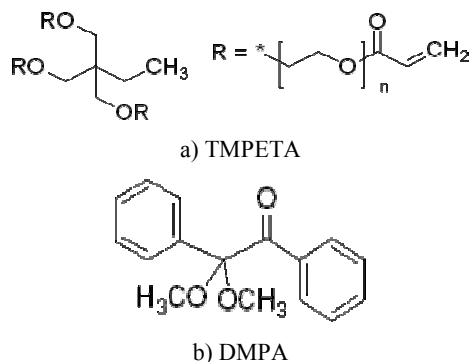
Fig. 1. Chemical structures of PHP I components
