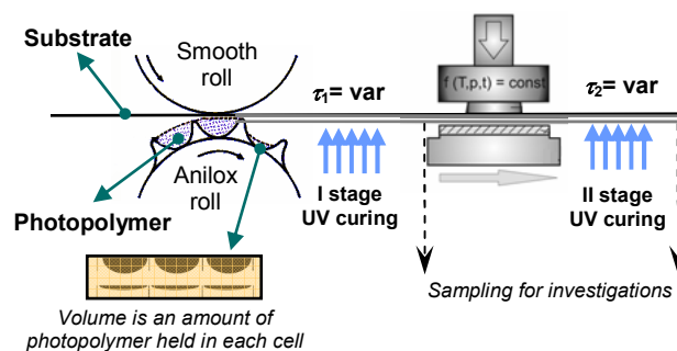
Fig. 2. Schematic view of photopolymer layer formation using two stages of UV curing
