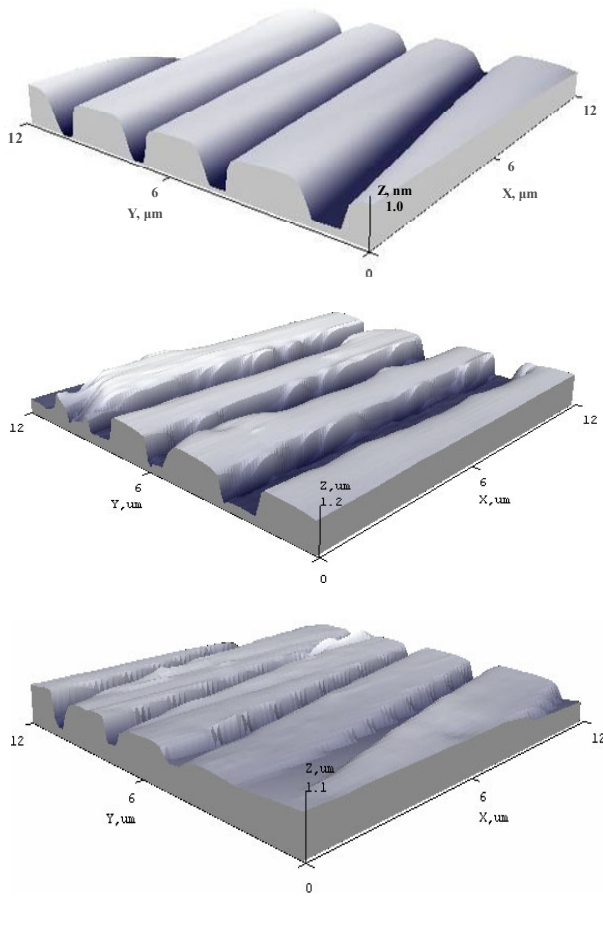
Fig. 7. AFM images and profiles of embossed periodical structures vs photopolymer type and effective initial UV curing duration \tau , s: a – PHP I (10 s); b – PHP II (20 s); c – PHP III (30 s)
