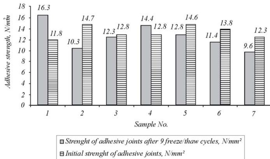
Fig. 10. Dependence of adhesive joint strength according to conditioning sequence No.2 on the amount of pure and crude glycerol and on freeze / thaw cycles
