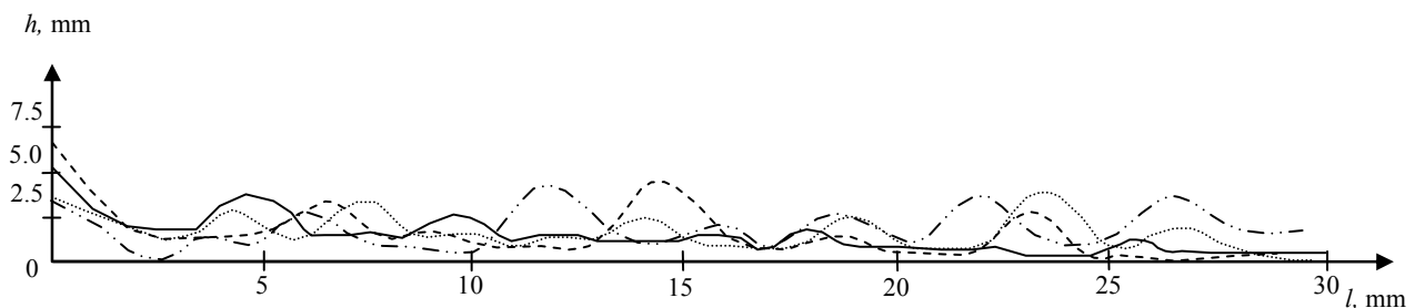
Fig. 1. The example of geometrical shape of assembled specimens cut from fabric F1 in warp direction, when pressing force 65 N and main shaft rotational frequency: 200 (—), 900 (.....), 1600 (---) and 2300 min -1 (-.-.-)
