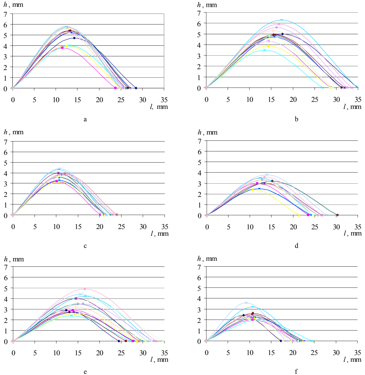
Fig. 3. (in colour on-line) Inherent waves in the fabrics F1 warp (a) and weft (b), F2 warp (c) and weft (d), F3 warp (e) and weft (f) directions when main shaft rotational frequency 200 min -1 and pressing force 25 N (—◆—), 45 N (—■—), 65 N (—▲—), 85 N (—✱—); main shaft rotational frequency 900 min -1 and pressing force 25 N (—✱—), 45 N (—◆—), 65 N (—▲—), 85 N (—■—), main shaft rotational frequency 1600 min -1 and pressing force 25 N (—▲—), 45 N (—✱—), 65 N (—■—), 85 N (—◆—); main shaft rotational frequency 2300 min -1 and pressing force 25 N (—◆—), 45 N (—✱—), 65 N (—■—), 85 N (—▲—)
