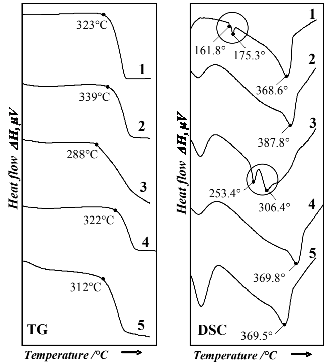
Fig. 2. TG and DSC curves of the investigated objects: 1 – polylactide; 2 – cotton; 3 – soybean protein; 4 – tencel; 5 – bamboo
