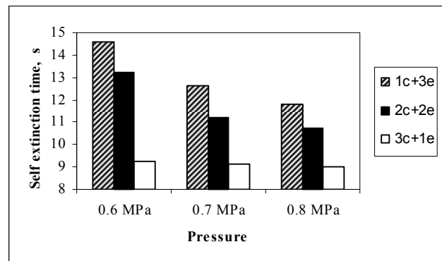
Fig. 7. Dependence of fabric self extinction time on air pressure in the texturing jet
