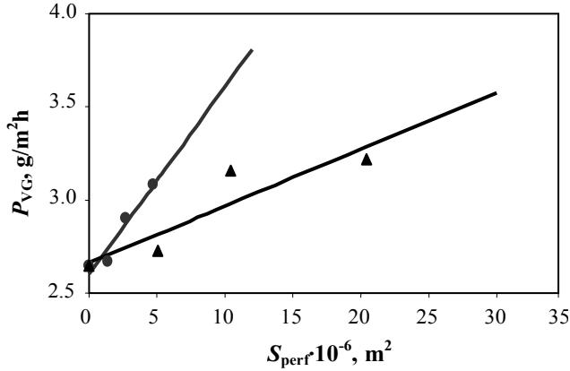
Fig. 2. Relation between the laminated leather water vapour permeability ( P_{VG} ) and the perforation area S_{perf} : ● – \rho_1 = 0.83 \text{ cm}^{-2} , ▲ – \rho_2 = 3.64 \text{ cm}^{-2}
