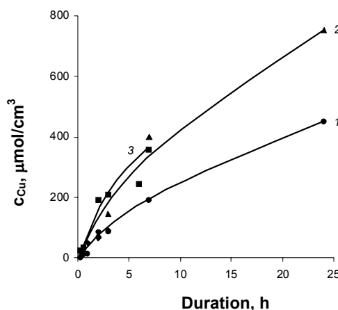
Fig. 3. Dependence of copper concentration in PA on chalcogenization duration when treating it with \text{Na}_2\text{TeS}_4\text{O}_6 solution at 20^\circ\text{C} and then in \text{Cu}(\text{II/I}) salt solution. The concentration of \text{Na}_2\text{TeS}_4\text{O}_6 solution, \text{mol}/\text{dm}^3 : 1 – 0.01; 2 – 0.025; 3 – 0.05
