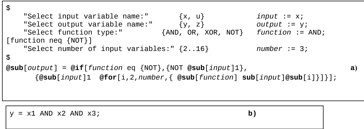
Figure 7. Encoding of FD given in Figure 3 using Open PROMOL (a); (b) one of derivative instances
