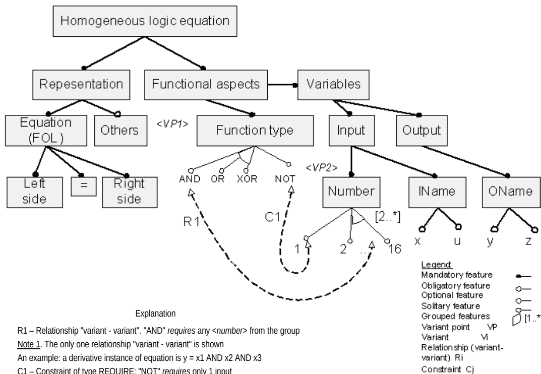
Figure 3. FD as a domain model instantiated from its meta-model
