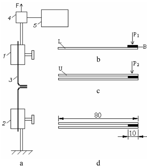
Fig. 1. The layout of „TINIUS OLSEN H10KT“ tension machine: 1 – upper grip, 2 – bottom grip, 3 – specimen, 4 – the sensor of force measurement, 5 – software equipment (a), adhesive film (B) transferring (b), bond of fabric layers (L and U) (c), parameters of specimen (d)
