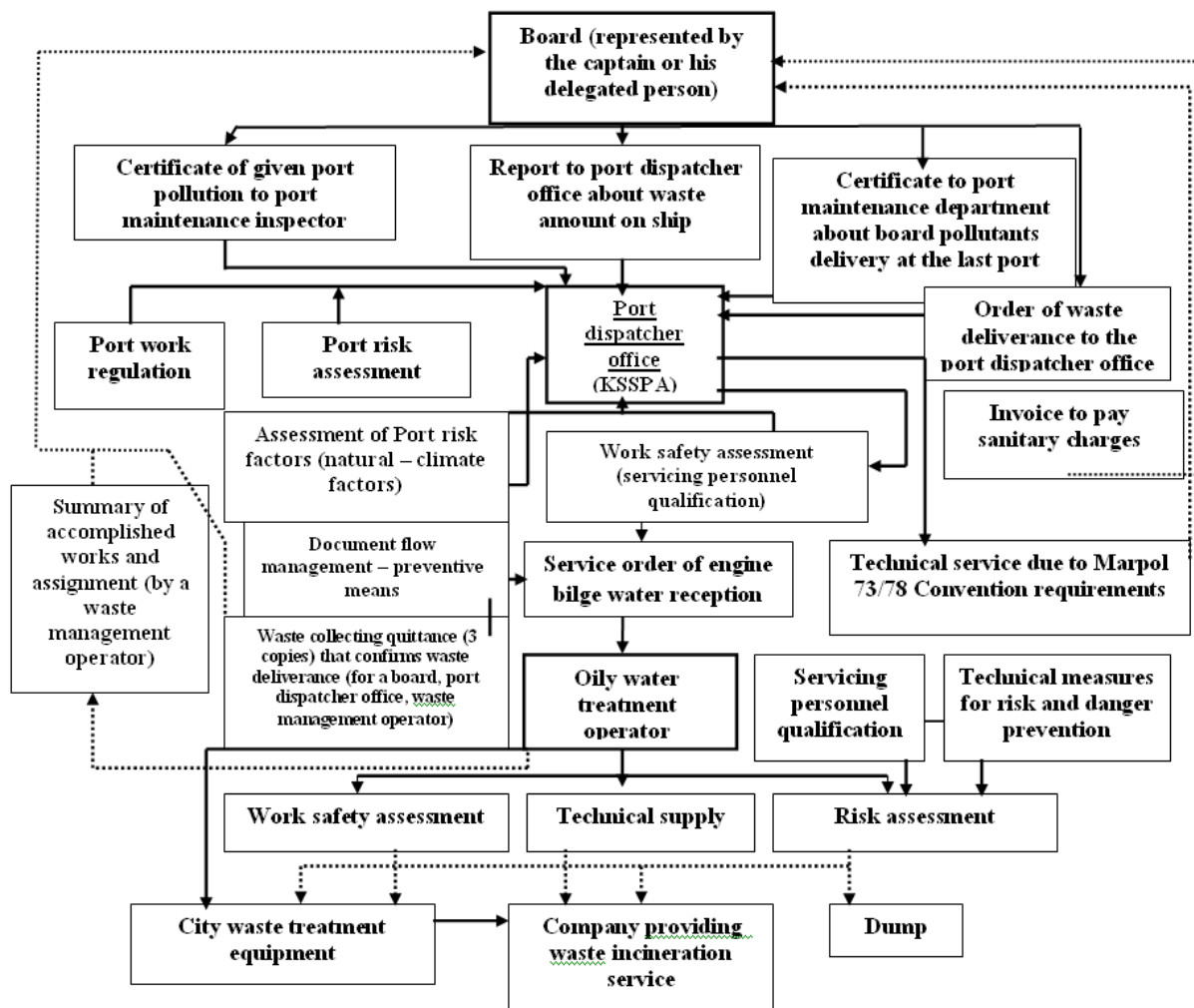
Chart 2. Information and document flow control in Klaipėda port
