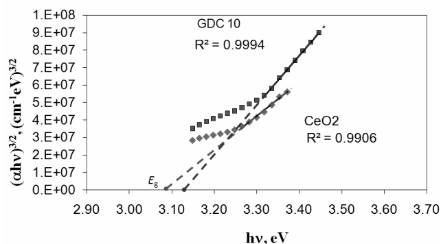
Fig. 7. Tauc's plot for \text{CeO}_2 and annealed \text{CeO}_2/\text{Gd}_2\text{O}_3 (GDC10) multilayer films produced on the glass substrates
