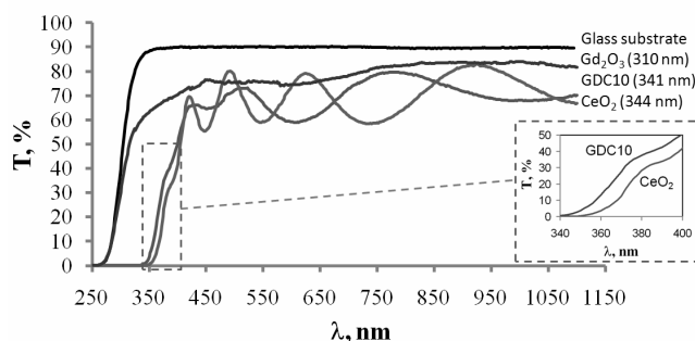
Fig. 6. Transmittance of \text{CeO}_2 , \text{Gd}_2\text{O}_3 films and \text{CeO}_2/\text{Gd}_2\text{O}_3 multilayer film annealed in 500 °C temperature. Thicknesses of the films are indicated in the graph
