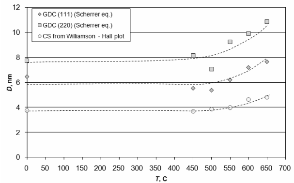
Fig. 5. Crystallite size of \text{CeO}_2/\text{Gd}_2\text{O}_3 multilayer thin films samples annealed in air atmosphere in temperatures from 450 °C to 650 °C
