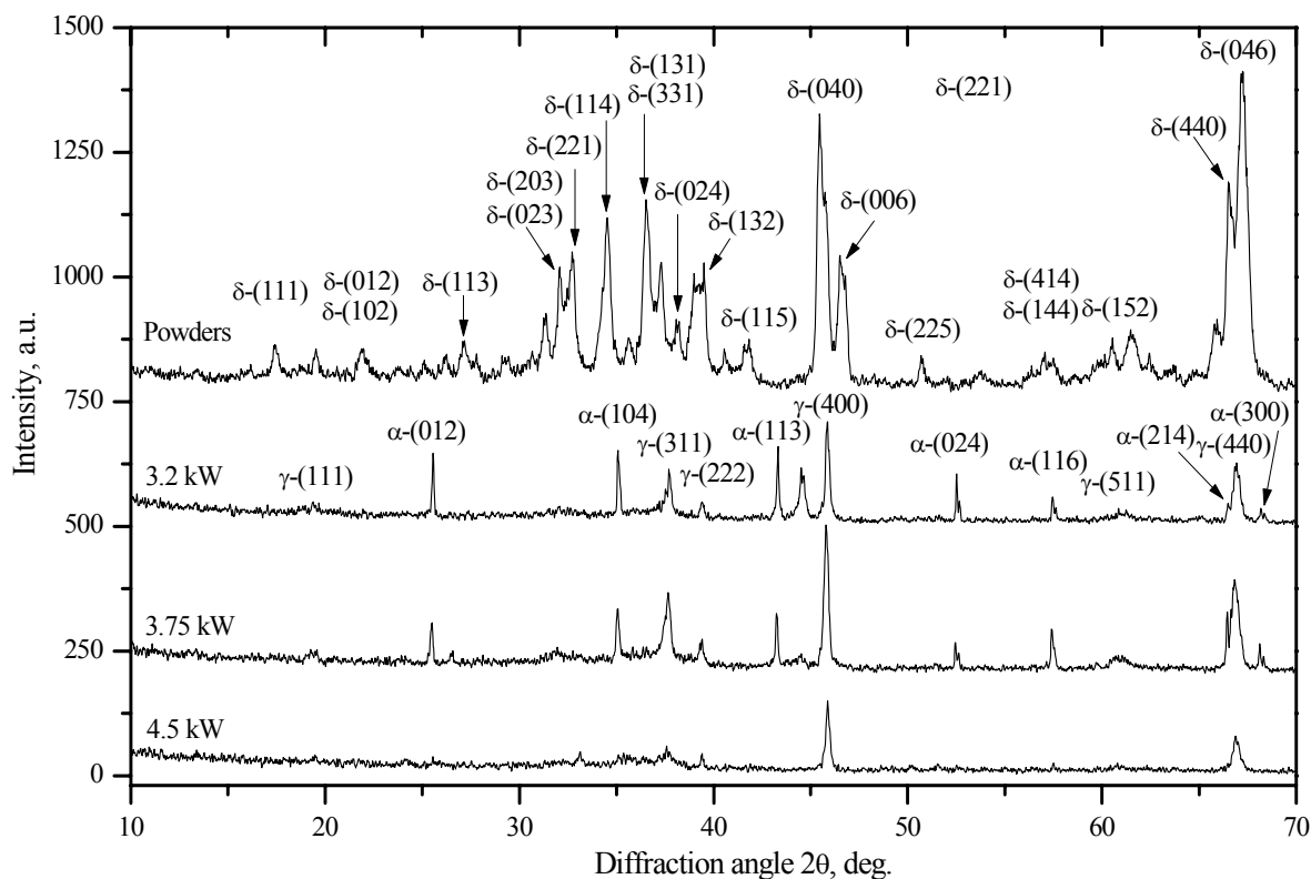
Fig. 3. XRD patterns of \text{Al}_2\text{O}_3 granules and coatings
