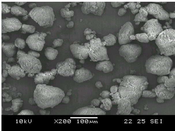
Fig. 1. SEM view of granulated \text{Al}_2\text{O}_3 powders
