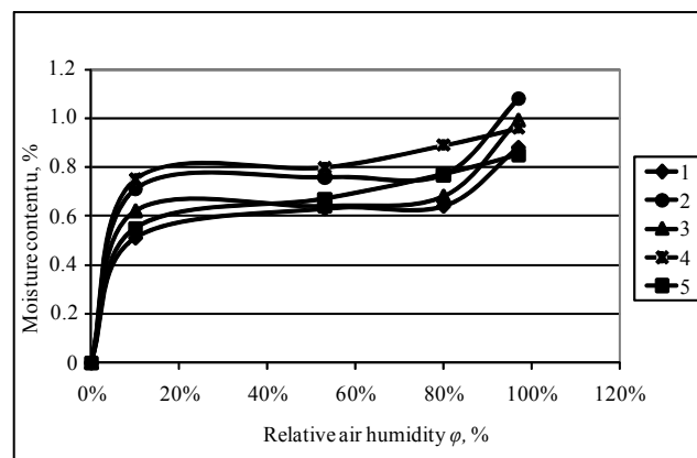
Fig. 3. The sorption curves of expanded polystyrene class EPS 80. 1–5 – sorption curves of products from different manufacturers'
