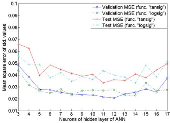
Figure 5. Selection of the number of neurons in the hidden layer of ANN and transfer function
