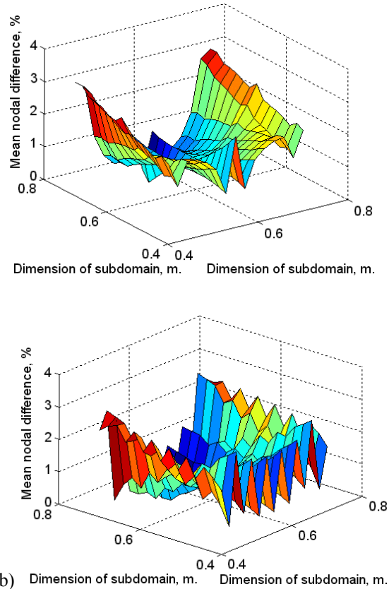
Figure 9. The estimated values of differences of displacements of the corresponding nodes of equivalent membrane (calculated by ANN) and girder by using test model, where a) N_m = 36 and b) N_m = 21
