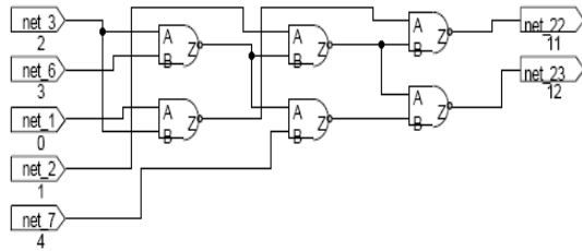
Figure 1. Circuit c17 from the benchmark suite ISCAS85
