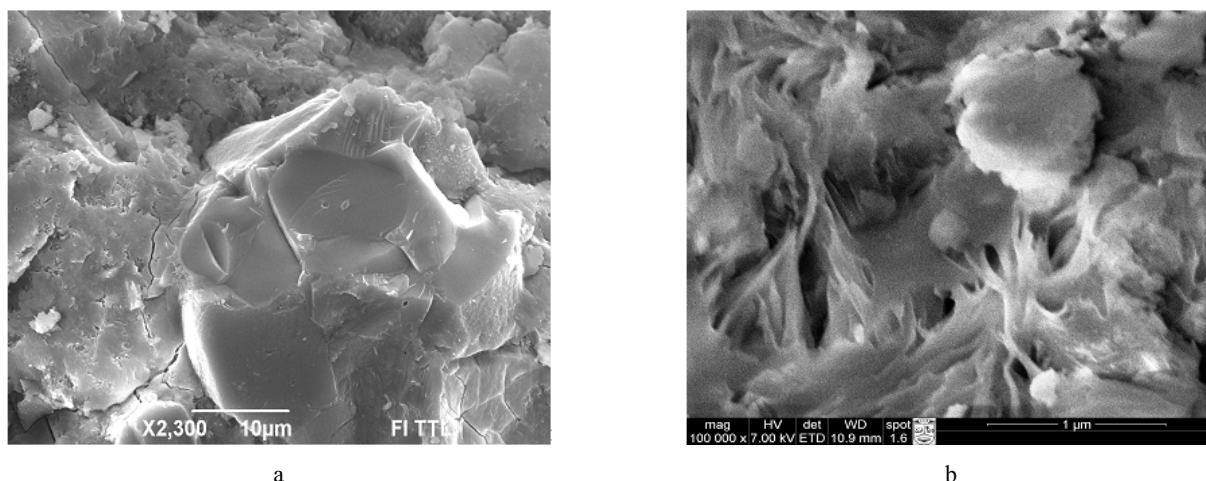
Fig. 3. Structure of aluminate cement stone: a – general view, b – minor crystalline hydrates
