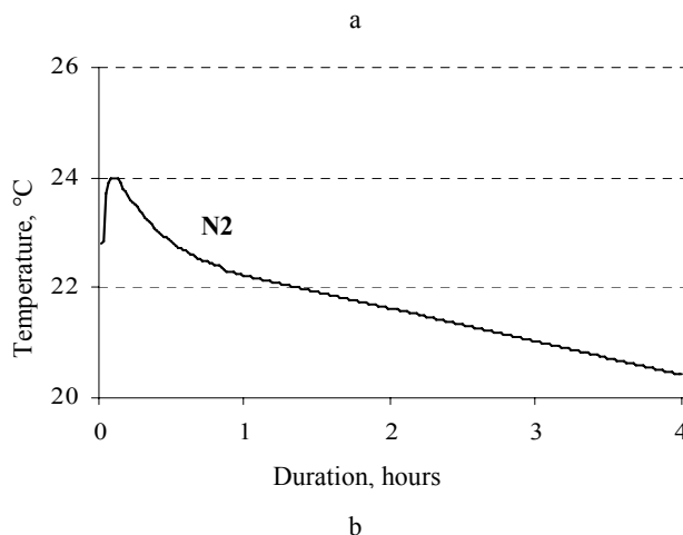
Fig. 2. Exothermal temperature during hardening of binders: a – composition N1 and N3, b – N2
