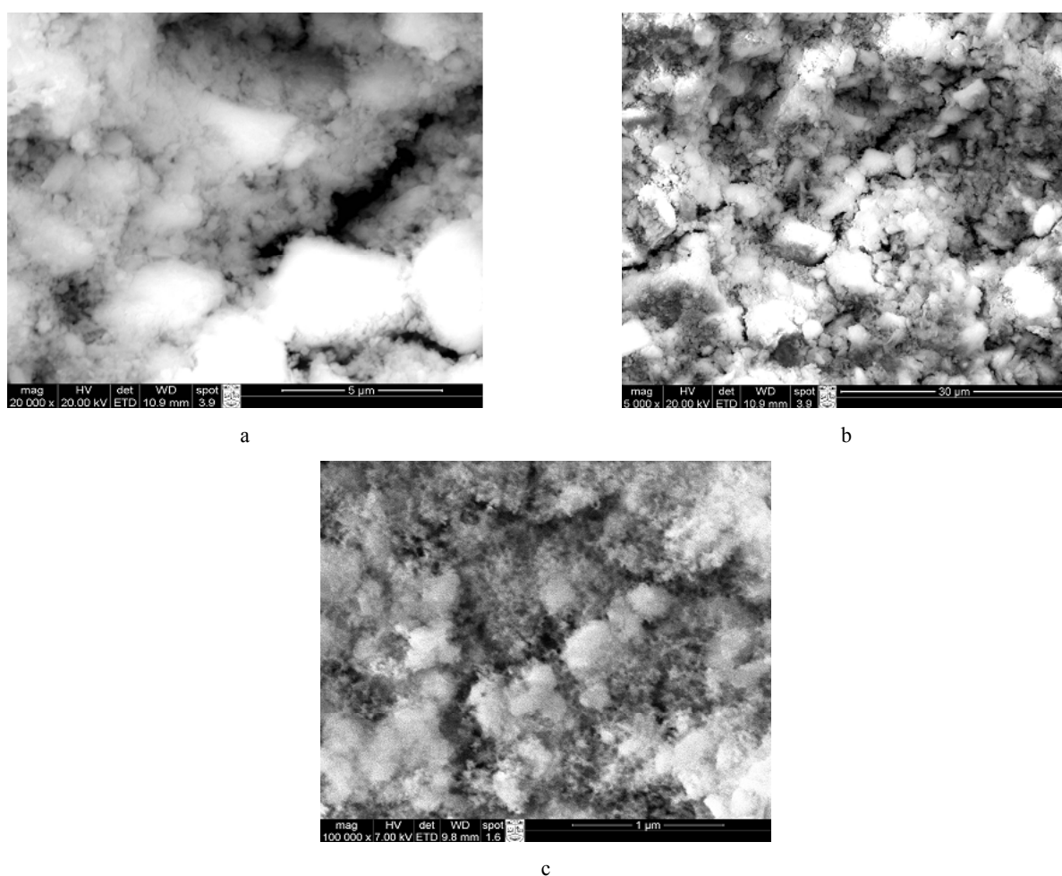
Fig. 4. Structure of liquid glass binder: a – magnification \times 5\,000 , b – \times 20\,000 , c – \times 100\,000
