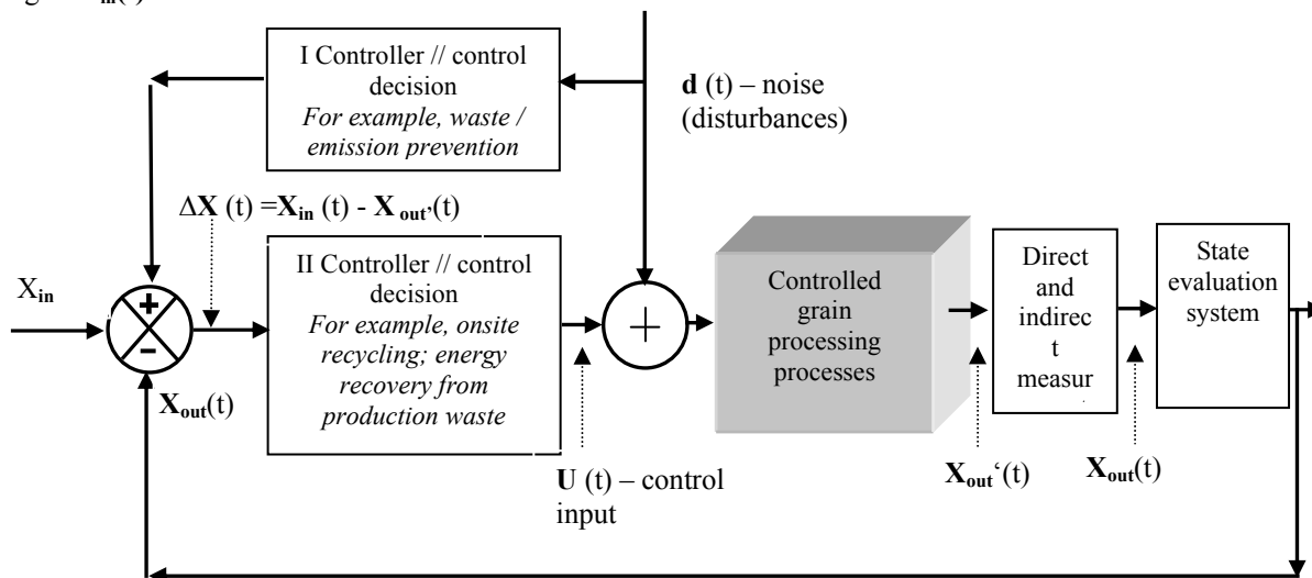
Fig. 4. Significant environmental aspects control system in grain processing
