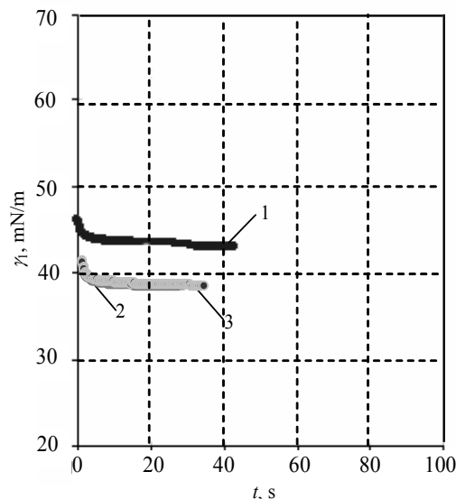
Fig. 5. The changes of resin solution ( C = 52\% ) surface tension \gamma_1 in time t vs \text{TiO}_2 content, phr: 1 – 2; 2 – 5; 3 – 7
