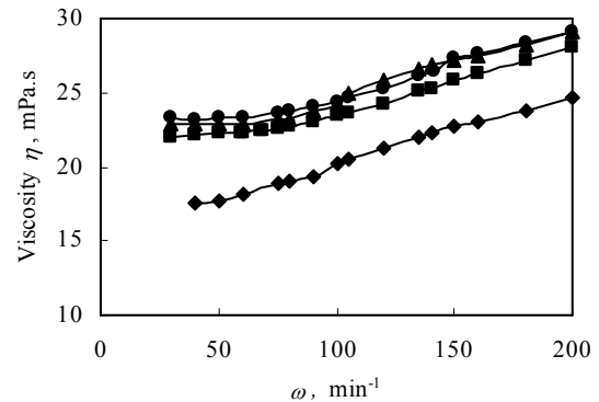
Fig. 3. Brookfield viscosity of resin solution at different rotational speed \omega vs \text{TiO}_2 content \phi , phr (♦ – 0, ■ – 2, ▲ – 5; ● – 7) at C = 52 % and T = 30 °C
